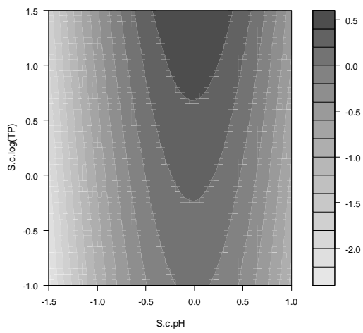
c) diatom genus richness
