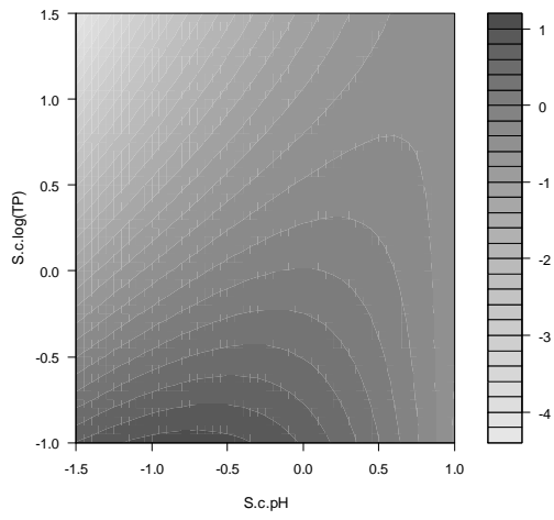
b) diatom taxon richness
