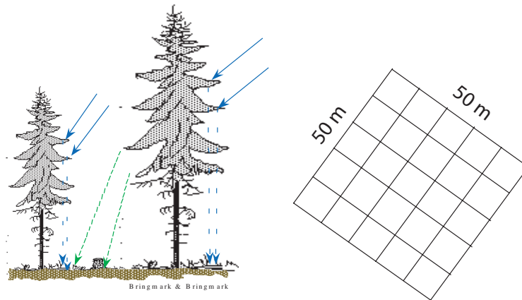
Fig. 2. Principles of sampling for spatial patterns in forest mor layers. Metals intercepted by trees were heterogeneously deposited on the forest floor directly as wet (blue lines) and dry deposition and after interception in the trees as throughfall and litterfall (green lines). Samples were taken at the nodes of regular grid systems measuring 50x50 m 2 .
