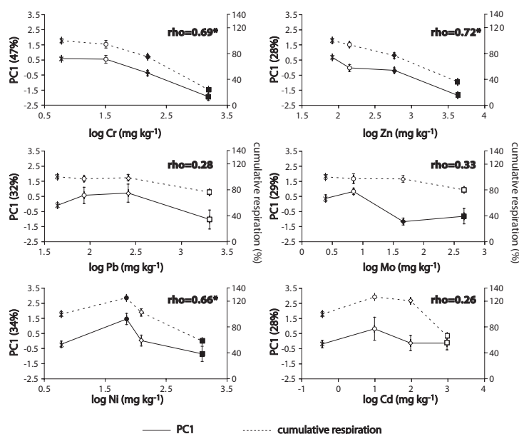
Fig. 9. Microbial community structure (sample scores of the first principal component (PC) of the PLFA pattern) and cumulative respiration as a function of heavy metal concentrations in experiments (logarithmic heavy metal concentrations for Cr, Zn, Pb, Mo, Ni, and Cd). Percentages on left axes indicate variation explained by PC1. Spearman rank correlation coefficients ( \rho ) between microbial community structure and cumulative respiration in all samples were calculated. Significant correlations are denoted *. Filled symbols differ significantly from controls (Anova, followed by Dunett's test for comparison with controls). Error bars in figures denote standard error (controls (x) n=12; low ( \circ ) n=4; medium ( \diamond ) n=4 and high dose level ( \square ) n=4). \alpha=0.05
