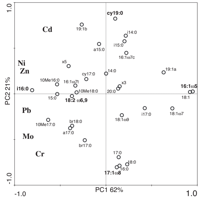
Fig.9. PCA based on loadings for the individual PLFAs from PC1 of separate RDA of each heavy metal (PC1 of RDAs accounted for 42%, 23%, 7%, 15%, 12% and 11% of the variation in the data set for Cr, Zn, Pb, Mo, Ni and Cd, respectively).
