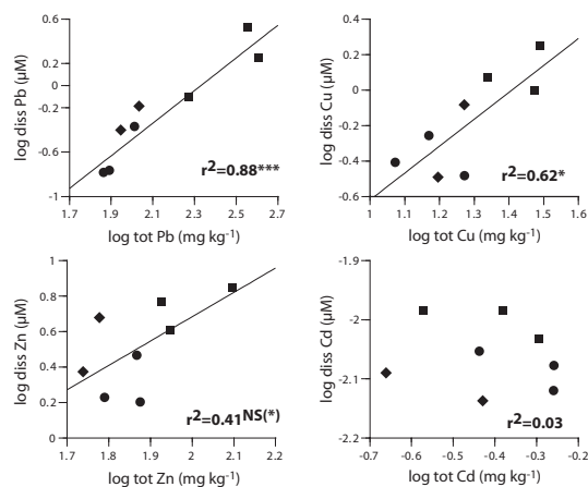
Fig. 4. Regression analysis between dissolved and total metal concentrations in bulk-samples at site 1 (■), site 2 (◆) and site 3 (●) m. Coefficient of determination ( R^2 ) between variables and levels of significance are denoted in the figures: * p < 0.05 , *** p < 0.001 . Not significant correlations are denoted NS.
