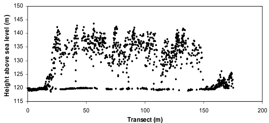
Fig. 6. Laser data from the airborne TopEye sensor acquired at a flight altitude of about 400 m above ground, with a pulse density of about 2.5 measurements per square meter. Each pulse is displayed as a black point plotted along a five meter wide transect through a forest stand (see Fig. 3).
