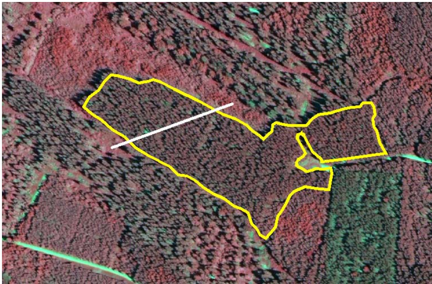
Fig. 3. A pansharpened color infrared image from the airborne Z/I DMC sensor acquired at a flight altitude of 4,800 m above ground, with a pixel size of 0.48 m. The imaged area covers about 600×400 m. The stand boundary, superimposed on the image, is outlined in yellow color. The white line shows the transect used to visualize laser data in Fig. 6.
