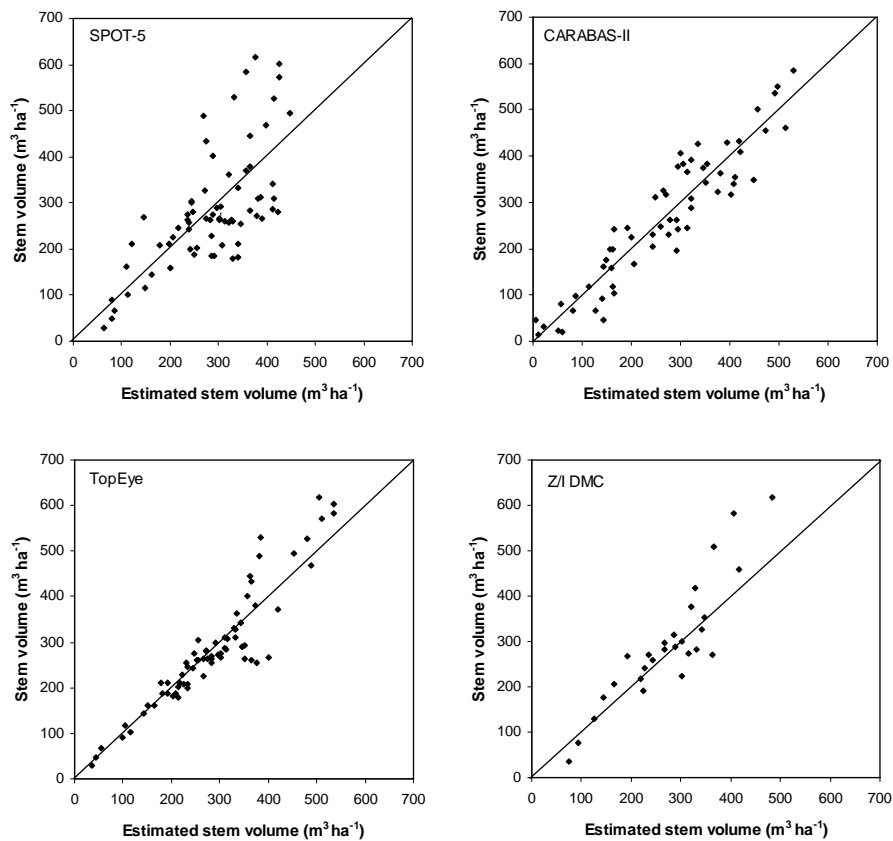
Fig. 8. Field measured stem volume plotted against estimated stem volume at stand level from single sensor data; SPOT-5 (paper V), CARABAS-II (papers I and II), TopEye (paper V), and Z/I DMC (paper III, Fig. 2 (B)) data. The plots are shown with reference lines.
