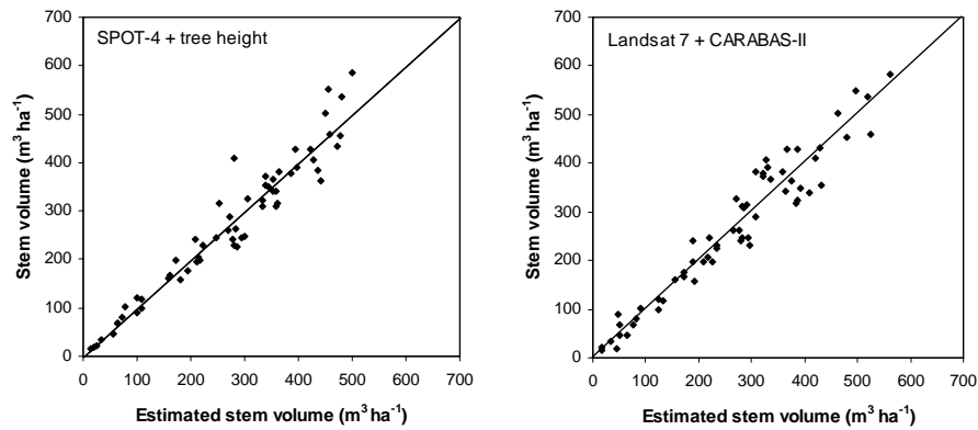
Fig. 9. Field measured stem volume plotted against estimated stem volume at stand level from combined sensor data; SPOT-4 and tree height (paper IV), Landsat 7 and CARABAS-II (paper II). The plots are shown with reference lines.
