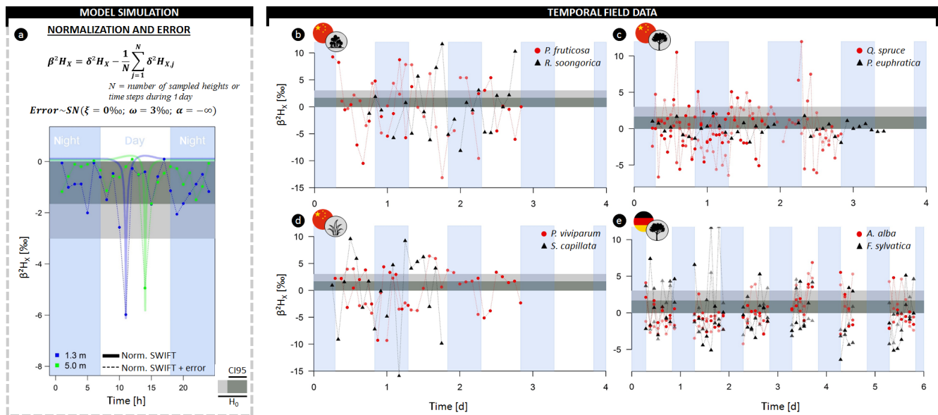
Figure 4. (a) Illustrative example of model simulations transformed in the normalized \delta^2\text{H}_X composition of xylem water ( \beta^2\text{H}_X ) at 1.3 (blue) and 5 m (green) sampling heights with the formula provided. Thicker lines indicate model simulations without error, and lines connected by dots indicate a scenario of hourly sampling with consideration of the extraction error (i.e., a negative skew normal distribution; \xi = 0\% , the scale \omega = 3\% , and shape \alpha = -\infty ). (b–e) High temporal field measurements of \beta^2\text{H}_X of (b) two shrubs, (c) two trees, and (d) two herb species sampled in the Heihe River Basin (northwestern China) and (e) two tree species sampled in the Freiamt field site in southwest Germany. The horizontal gray-colored envelope in all panels delineates the acceptable variance from the stem mean according to the null model ( H_0 ), i.e., assuming no variance along the length of a lignified plant aside from the potential extraction error (i.e., 3%). Herein, the dark gray envelope indicates the confidence interval comprising 95 % of potential extraction error (CI95). A breakdown of the field data on species and individual level is provided in the Supplement figures (Figs. S3–S6).
