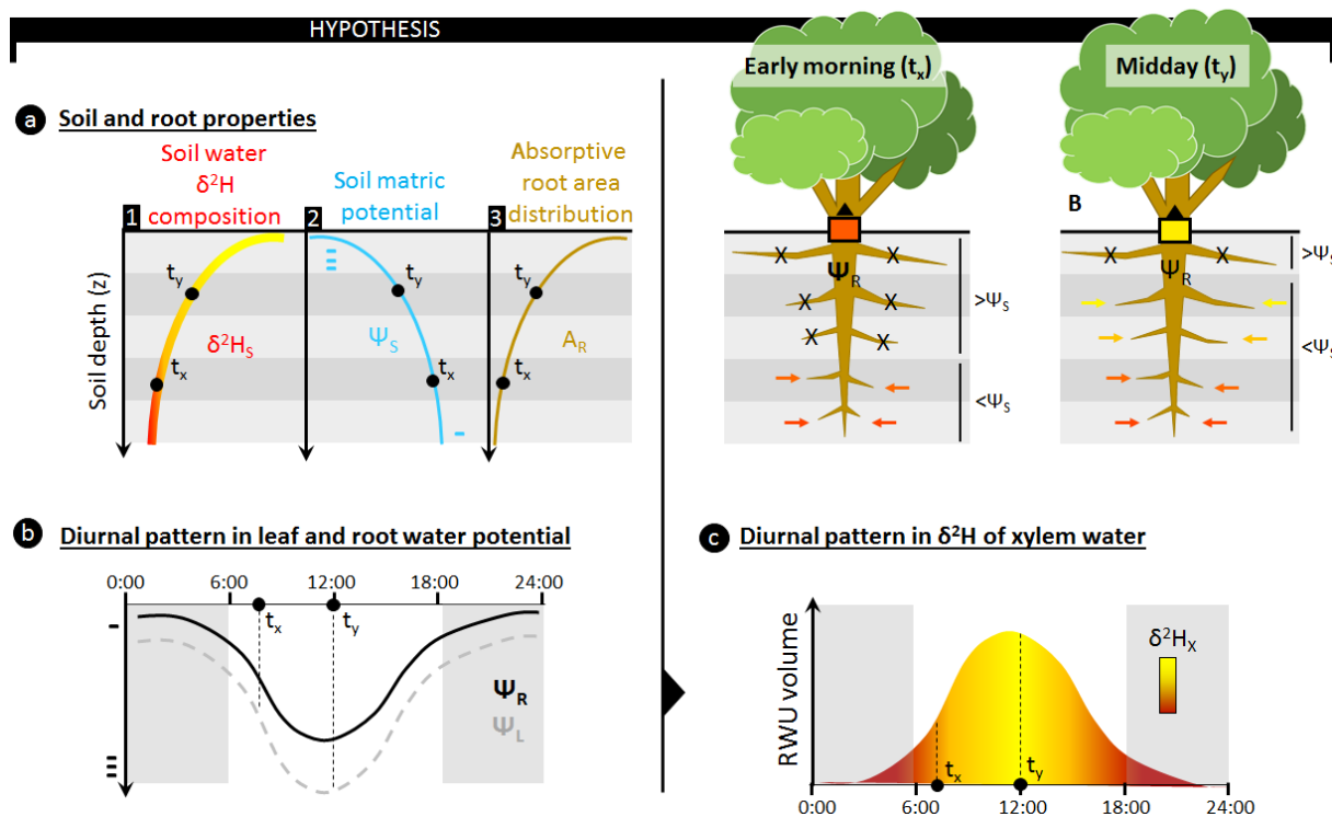
Figure 1. The use of stable water isotopes ( \delta^2\text{H} and \delta^{18}\text{O} ) to assess the relative depth of root water uptake (RWU) requires a depth gradient in isotopic composition of soil water ( \delta^2\text{H}_S ) to be present (a, sub-panel 1) as only then can the relative contribution of different soil layers to the isotopic composition in a plant's xylem water ( \delta^2\text{H}_X ) be derived. These \delta^2\text{H}_S gradients occur naturally as the result of evaporative soil drying during drought conditions; however, these conditions also result in the formation of a gradient in soil matric potential ( \Psi_S ), ensuring an increasing \Psi_S with depth (a, sub-panel 2). RWU and sap flow in plants are passive processes in which water flows in the direction of decreasing water potentials. Specifically for RWU, this implies that water influx through the absorptive root area ( A_R ; a, sub-panel 3) of a plant's root is facilitated whenever the water potential in the root ( \Psi_R ) is more negative than the surrounding \Psi_S . As A_R and \Psi_S are generally not uniform with soil depth ( z ), the relative contribution of a specific soil layer to RWU will depend on (i) the difference between \Psi_S and \Psi_R in that soil layer and (ii) the relative amount of absorptive root area in that soil layer. Stable water isotope techniques assume that the \delta^2\text{H}_X reflects the contribution of \delta^2\text{H}_S from all soil layers. However, this does not account for the diurnal fluctuations in \Psi_R which are invoked by the diurnal patterns in a plant's transpiratory water demands (b). Typically, more negative \Psi_R values are observed when water demands are high, i.e., around midday. However, a decrease in \Psi_R will result in higher RWU and alter the contribution of different soil layers to RWU. Specifically, dryer and shallower soil layers, with more negative \Psi_S , could start contributing to RWU as \Psi_R decreases (c). For example, in the early morning (situation t_x ) when \Psi_R is high, only deeper soil layers where \Psi_S is greater than \Psi_R contribute to the overall \delta^2\text{H} composition of the RWU flux. As \Psi_L and \Psi_R decrease towards midday (situation t_y ), more water can be absorbed from shallower soil layers. As the A_R in these shallow soil layers is high, they strongly affect the relative contribution of \delta^2\text{H}_S entering the plant. Hence, diurnal fluctuations in \Psi_R will result in fluctuating mixtures of \delta^2\text{H}_S entering the plant. As these \delta^2\text{H}_S mixtures are transported along the xylem pathway, they produce variances in \delta^2\text{H}_X which could complicate RWU assessments via stable water isotope analysis.
