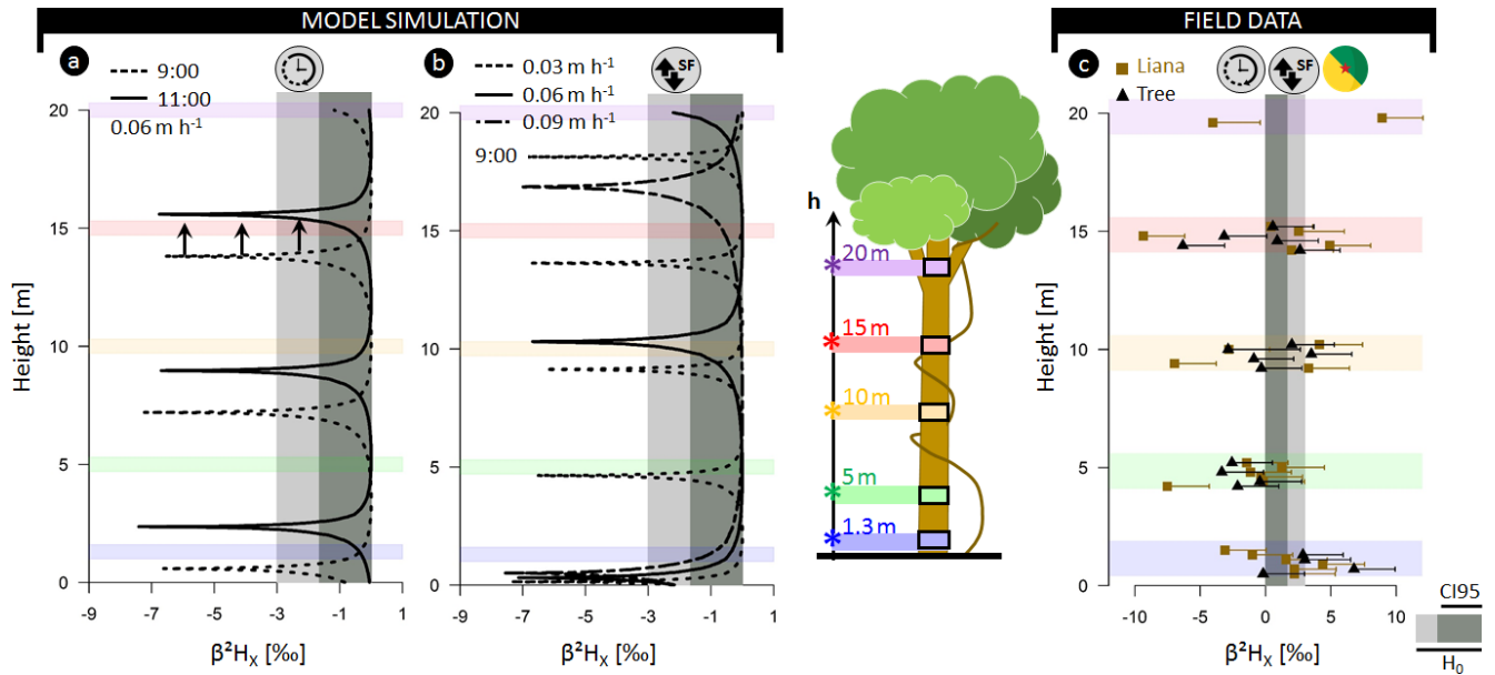
Figure 3. (a) Model outputs for model analysis A3 representing the normalized \delta^2\text{H} composition of xylem water ( \beta^2\text{H}_X ) as a function of the tree height simulated for different sampling times (09:00 and 11:00). The modeled tree has an average daily sap flux density of 0.06\text{ m h}^{-1} ( \text{SF}_S ; approximate daily true sap flux density \text{SF}_V = 0.42\text{ m h}^{-1} ). (a) Model outputs for model analysis B where \beta^2\text{H}_X in relation to stem height is shown at 09:00 LT but parameterized with distinct \text{SF}_S , i.e., 0.09 , 0.06 , and 0.03\text{ m h}^{-1} (corresponding to \text{SF}_V values of 0.64 , 0.42 , and 0.19\text{ m h}^{-1} , respectively). The standard parameterization used for both study analyses is detailed in Table S1. (c) Field measurements of \beta^2\text{H}_X for six lianas (■) and six trees (▲). Error whiskers are the combination of potential extraction and measurement errors of the isotope analyzer. A species-specific breakdown of the field data is provided in Fig. S2. The horizontal gray-colored envelope in all panels delineates the acceptable variance from the stem mean according to the null model ( H_0 ), i.e., assuming no variance along the length of a lignified plant aside from the potential extraction error (i.e., 3\% ). Herein, the dark gray envelope indicates the confidence interval comprising 95% of potential extraction error (CI95).
