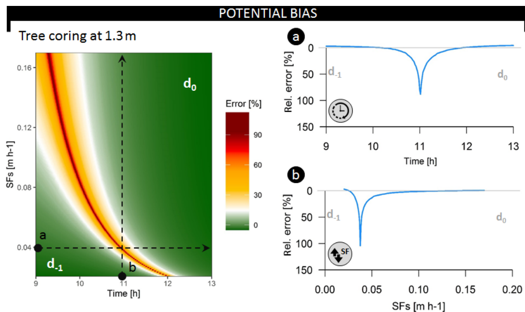
Figure 5. Relative error on the inferred average root water uptake depth (i.e., bias between the average daily and the instantaneously derived average RWU depth) at a coring height of 1.3 m throughout the common sampling period (09:00 until 13:00) and over a range of potential SF_S values (in m\ h^{-1} ), corresponding to an SF_V range of 0.15\text{--}1.25\ m\ h^{-1} . Both dotted lines describe test scenarios evaluated in the breakup panels. Respectively, d_{-1} and d_0 indicate whether the derived average RWU depth error corresponds to the previous or current day of measurement. The dynamics in relative error are when sampling (a) over different time steps and restricting sap flux density at 0.04\ m\ h^{-1} (i.e., SF_V = 0.28\ m\ h^{-1} ) or (b) over different SF_S values when restricting sampling time to 11:00 LT each day.
