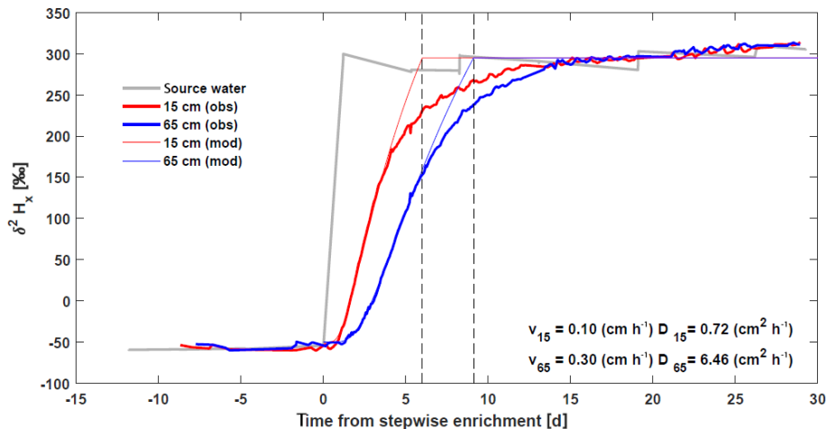
Figure 6. Basic model validation comparing continuous in situ \delta^2\text{H}_x measurements of a stepwise ^2\text{H} enrichment experiment (Marshall et al., 2020) with analytical solutions of an advection–diffusion equation at heights 0.15 m (—) and 0.65 m (—) on a pine tree ( Pinus pinea L.). The source water of the intact-root, isotopic-enrichment greenhouse experiment is presented in gray. Model parameters, velocity, and diffusion were fitted by visual inspection independently for the two heights to match the initial increase in isotope signature (values reported in the bottom right).
