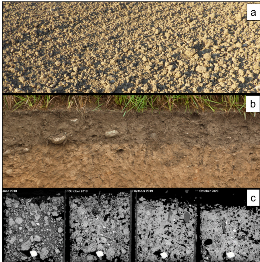
Figure 2. Aggregates are clearly visible following tillage in topsoils but are indistinguishable at deeper soil horizons and over time. (a) Aggregates are clearly evident in a freshly tilled soil (photo by Dani Or, ETH Zurich, Switzerland) but are not visible in (b) deeper soil layers of undisturbed soils at the same spatial scale. (c) The temporal evolution of soil structure after tillage based on X-ray computed tomography images (visible pores > 120 \mu\text{m} , based on voxel size of 60 \mu\text{m} ): aggregates are clearly visible directly after tillage (left panel, June 2018) but coalesce and fuse with time (right panel, October 2020) (John Koestel, unpublished).
