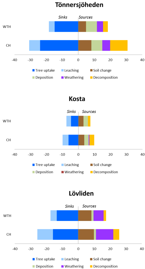
Figure 2. MAGIC modelled \text{Ca}^{2+} fluxes ( \text{kmol}_c \text{ha}^{-1} ) in CH- and WTH-plots summarized over the period 1990-2013 (Tönnersjöheden), 1991-2012 (Kosta) and 1991-2013 (Lövliden). The fluxes are divided into sinks (uptake, leaching) and sources (deposition, weathering, decomposition, soil change).
