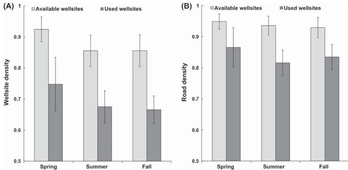
Figure 3. (A) Mean surrounding wellsites density (wellsites km -2 ), and (B) mean surrounding road density (km road km -2 ) for available versus used wellsites, by season in west-central Alberta, Canada, 2006–2012. Error bars represent standard error (SE).
