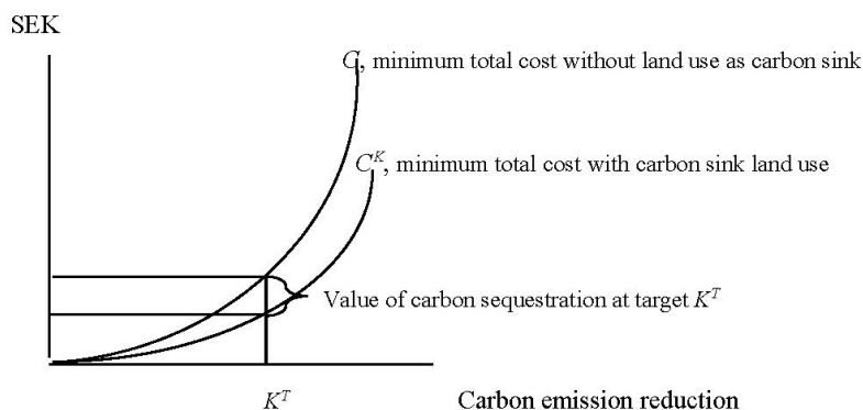
Figure 1. Illustration of the calculation of the value of land use as a carbon sink in a cost effectiveness framework. SEK: Swedish crown; K^T : carbon emission reduction target.
