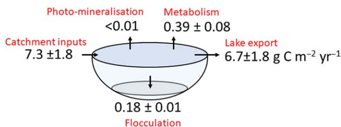
Fig. 4. Carbon budget of lake in \text{g C m}^{-2} catchment \text{yr}^{-1} . DOC inputs, DOC outputs, and lake DOC retention in annual mean \pm standard deviations (1986–2015). Lake DOC retention (modeled) partitioned into three processes of carbon removal from water phase: (1) microbial metabolism, (2) flocculation, and (3) photo-mineralization.
