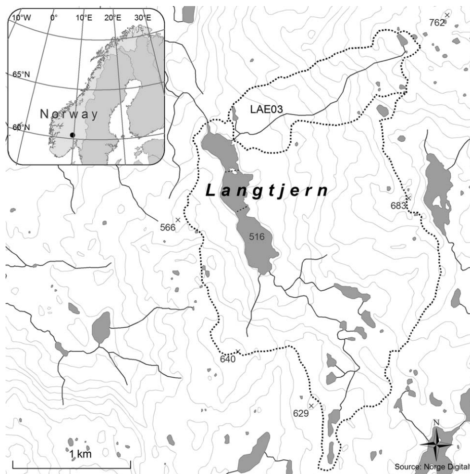
Fig. 1. The Langtjern lake catchment and its position in Norway. Subcatchment LAE03 to the east. The boarder between the three lake basins indicated by dotted line.
