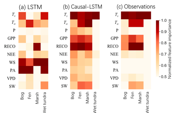
Fig. 4. Comparison of feature importance in (a) LSTM, (b) causal-LSTM, and (c) observations. Colors show the corresponding normalized feature importance that is normalized between 0 and 1, with higher value indicating higher importance.
