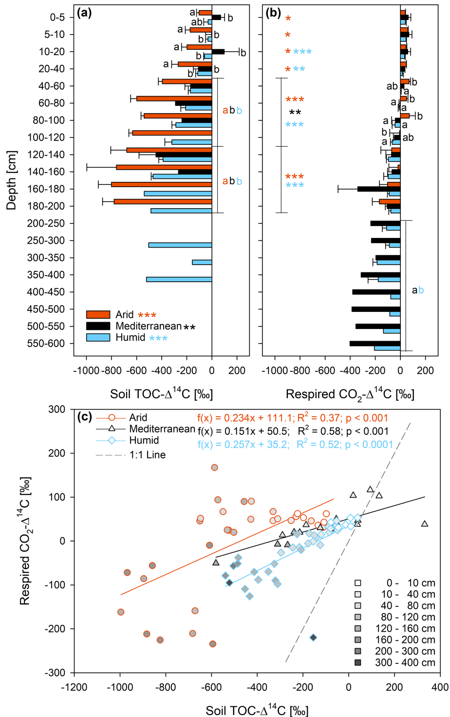
Figure 2. Radiocarbon ratio ( \Delta^{14}\text{C} ; mean \pm standard error) of (a) soil total organic carbon (TOC) and (b) respired \text{CO}_2 -C as well as (c) their relationship in soils at three sites (arid, mediterranean, humid) located along a precipitation gradient in the Coastal Cordillera of Chile (0–200 cm: n = 3 , except for humid site with n = 4 ; > 200 cm: n = 1 , except for humid site 200–400 cm with n = 2 ). Different letters in (a) and (b) indicate significant differences ( p \leq 0.05 ) among the sites tested by Tukey's post hoc test after two-way ANOVA. Asterisks indicate significant differences between the radiocarbon ratio of the total soil organic carbon (TOC) and that of the respired \text{CO}_2 -C for each site, tested across all soil depth increments (see legend) and also separately for the different sites and depth increments (* p \leq 0.05 , ** p \leq 0.01 , *** p \leq 0.001 ). The colors of the asterisks indicate the site the asterisks refer to. Lines in (a) and (b) indicate which soil depth increments were combined (separately per site) for statistical analysis.
