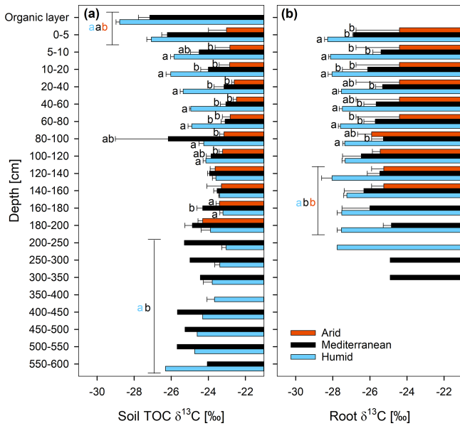
Figure 3. ^{13}\text{C} ratio ( \delta^{13}\text{C} ; mean \pm standard error) of (a) soil total organic carbon (TOC) and (b) roots at three sites (arid, mediterranean, humid) located along a precipitation gradient in the Coastal Cordillera of Chile (0–200 cm: n = 3 , except for humid site with n = 4 ; 200–600 cm: n = 1 , except for humid site 200–400 cm with n = 2 ). Different letters in (a) and (b) indicate significant differences ( p \leq 0.05 ) among the sites tested by Tukey’s post hoc test after two-way ANOVA. Lines in (a) and (b) indicate which soil depth increments were combined (separately per site) for statistical analysis.
