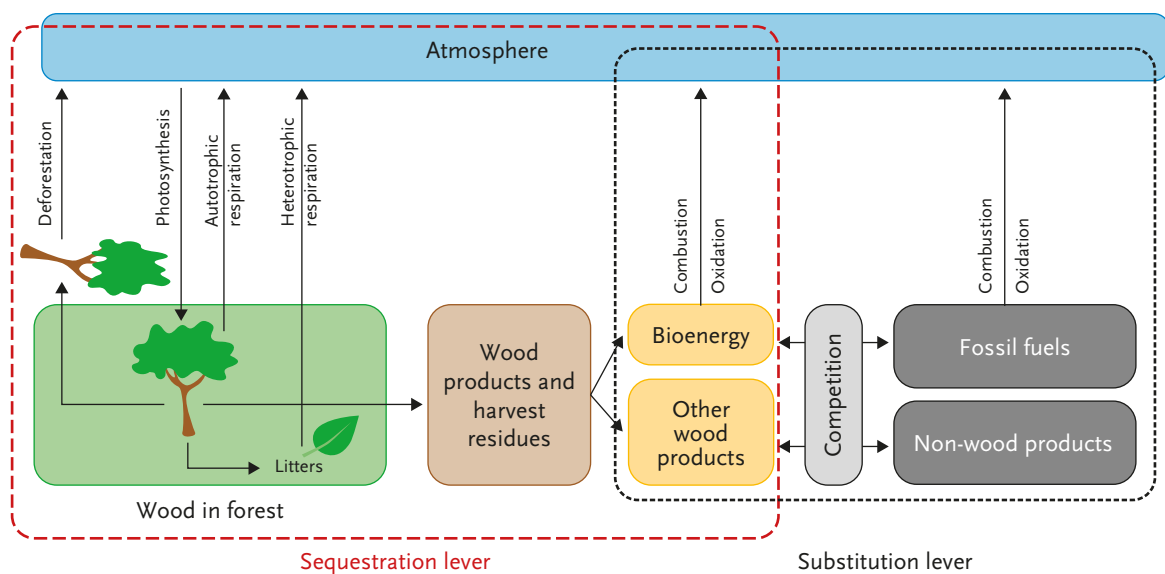
Figure 2. Simplified diagram of carbon stocks in reservoirs and flows between the atmosphere, biosphere and fossil reservoir. The two mitigation levers are depicted here.
