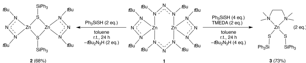
Scheme 2 Reaction of 1 with 2 and 4 equivalents of triphenylsilanethiol to give 2 and 3 , respectively.
