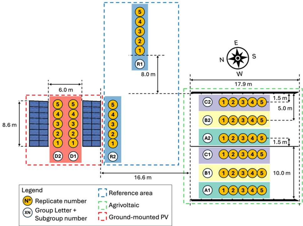
Fig. 1. Crop experiment layout (top view) of the vertical agrivoltaic system and conventional ground-mounted system in Kårbo Prästgård, Sweden. The illustration is not to scale.
