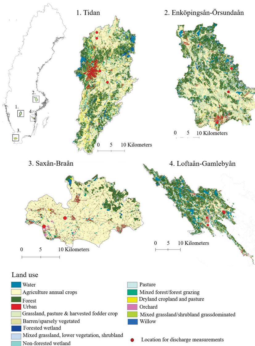
Figure 5. Location and land use of the four catchments used in methodological approach ( Paper I ) hydrological modelling of historical landscape ( Paper II , catchment no.1, Tidan) and Paper III (catchments no. 1-4, Tidan, Enköpingsån-Örsundaån, Saxån-Braån and Loftaån-Gamlebyån). Adapted from Malmquist & Barron (2024).
