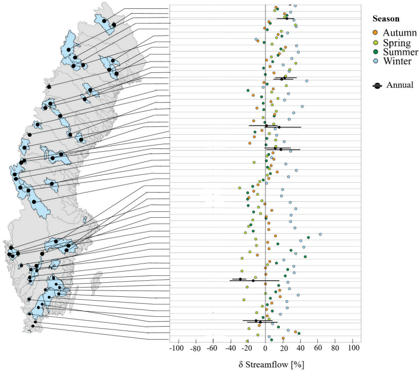
Figure 2. Observations (comparing 1961-1990 to 1991-2020) of historical change in average streamflow in Sweden. Black lines represent intervals over maximum and minimum changes over the measurement periods, Black dots represent annual average, coloured dots show seasonal (winter = blue, autumn = orange, spring = light green and summer = dark green) change between measurement periods. Values are extracted from Deutschbein et al. (2022) and Andréasson, (2004).
