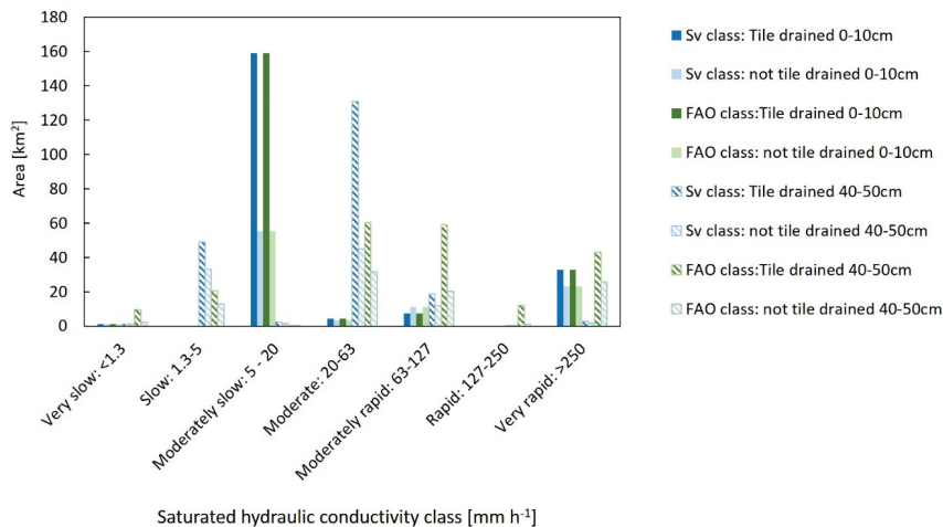
Figure S 2. Saturated hydraulic conductivity in field with (dark shade) - and without (light shaded color) identified tile drainage plans. Striped columns represent subsoil layers 40-50 cm
