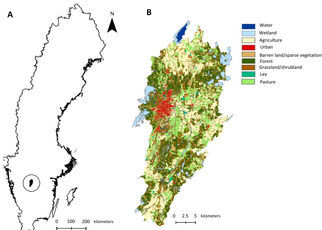
Fig. 1. Location of the study catchment, Tidan catchment (in the circle) (58.6 N, 14.0 E/58.2 N, 13.9 E) (A) and land use map of Tidan catchment for year 2020 with major land use classes (B).
