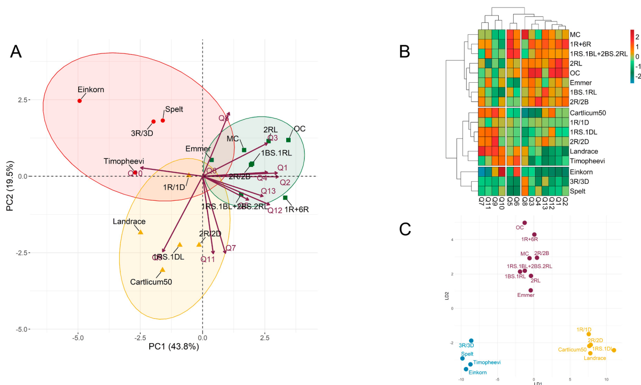
Fig. 3. Multivariate analysis of sensory attributes across 17 wheat genotype groups. (A) Contribution of the first two principal components (PC1 and PC2) explaining the variation among genotypes and 13 sensory traits. (B) Two-dimensional heatmap dendrogram displaying the clustering of genotype groups (rows) and 13 sensory attributes (columns) based on Z-score standardisation. (C) Linear discriminant analysis (LDA) of genotype groups, showing differentiation based on sensory profiles. Sensory traits include: Q1 – O-Graham flour (wet); Q2 – O-Rye flour; Q3 – O—Corn (raw); Q4 – O—Cooked rice (white); Q5 – A-Gray; Q6 – A-Beige; Q7 – TM-Grittiness (sandy); Q8 – TM-Sturdiness/Compact; Q9 – T-Umami; Q10 – T-Sweetness; Q11 – T-Bitterness; Q12 – F-Graham flour; Q13 – F-Rye flour.
