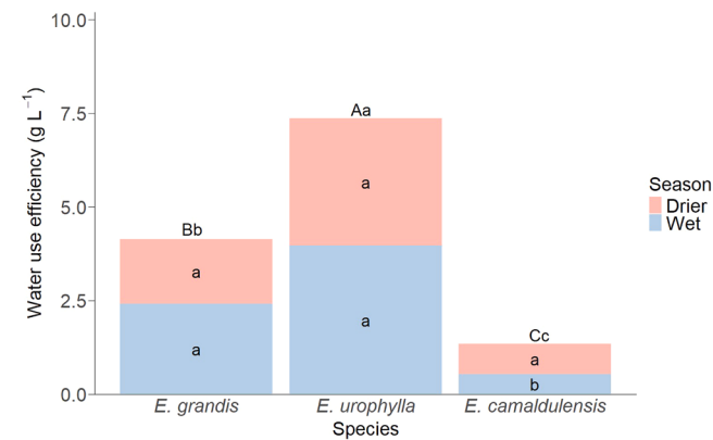
Fig. 13. Tree-level water use efficiency (WUE; stem biomass/transpired water) for each Eucalyptus species during the drier season (April to September) and the rainy season (October to March). Letters within the columns compare WUE between the two seasons for each species. Uppercase letters above the columns represent comparisons among species during the rainy season, while lowercase letters represent comparisons during the drier season. Columns followed by the same letter do not differ significantly according to the Kruskal-Wallis test with Bonferroni correction (Wilcox test) at p = 0.05 .
