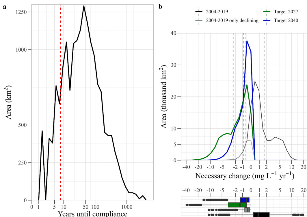
Fig. 8. a) Distribution of the time required until hotspots with declining trends in 2019 can comply with the water quality goal of 50 mg L -1 . The red dotted line represents the years until 2027. b) We explored the distribution of necessary changes that all hotspots in 2019 require to meet the water quality goal by 2027 and 2040. We also included the distribution of recent declining (grey) and all trends (black) for the period 2004–2019. Both a) and b) use a pseudo logarithmic scale in the x axis. (For interpretation of the references to colour in this figure legend, the reader is referred to the Web version of this article.)
