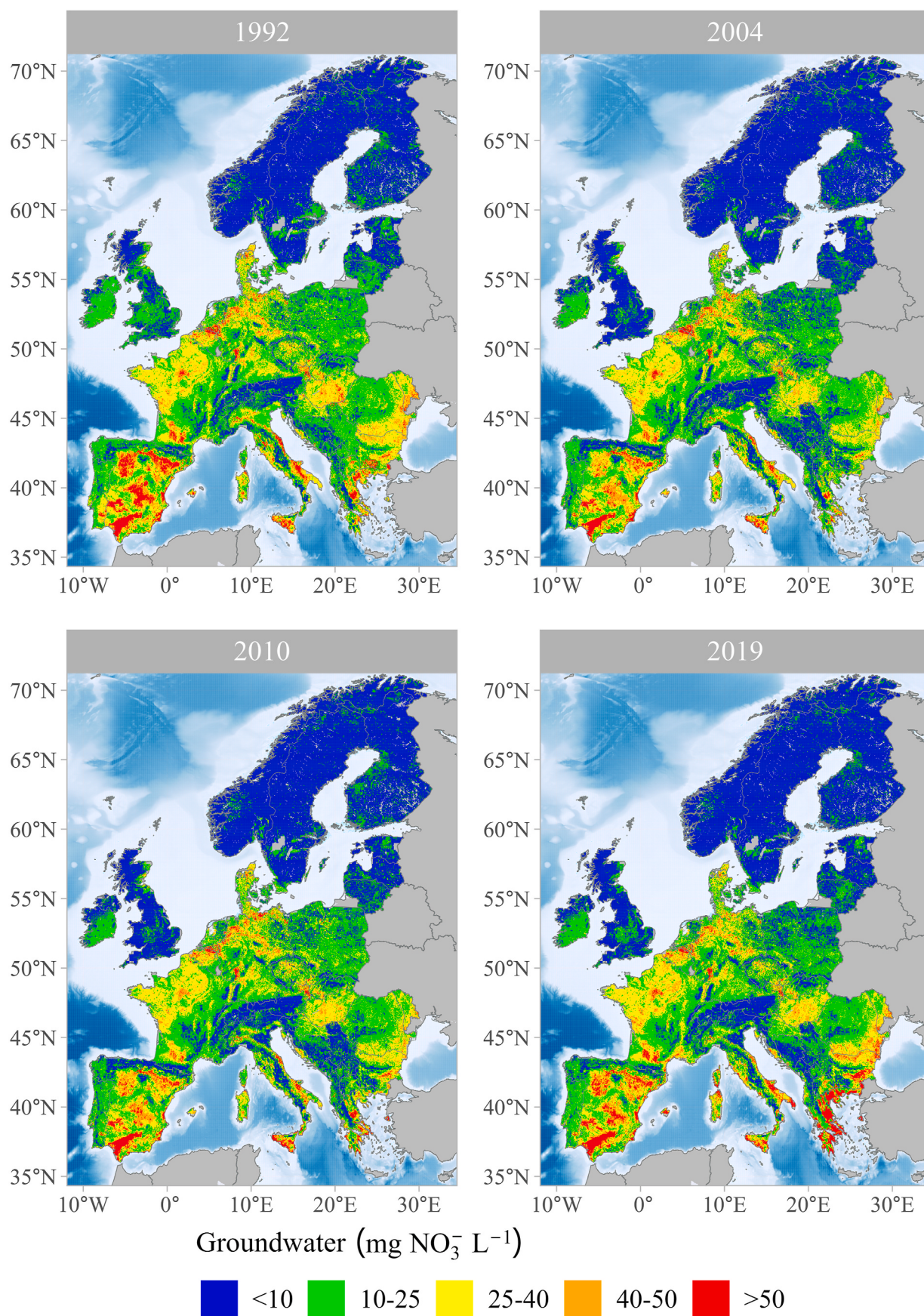
Fig. 3. Groundwater nitrate concentration predicted for snapshot years in Europe at 0.04^\circ \times 0.04^\circ . Hotspots, defined as concentrations above 50 \text{ mg L}^{-1} , according to the Nitrates Directive, are highlighted in red. (For interpretation of the references to colour in this figure legend, the reader is referred to the Web version of this article.)
