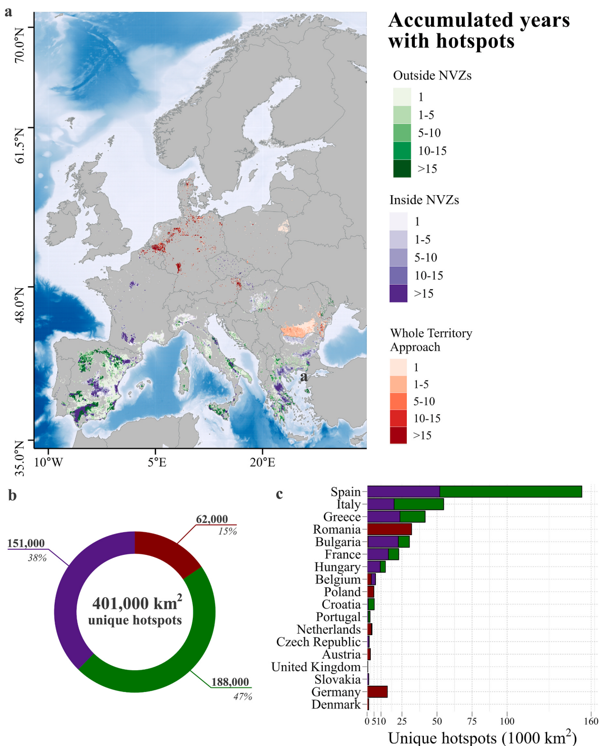
Fig. 5. a) Spatial variation of total accumulated hotspots over Europe during the period 1992–2019. b) and c) showcase the total accumulated hotspots at the European and national levels, respectively. Three spatial units were used: inside the NVZs, outside the NVZs and whole territory approach. The numbers refer to the sum of years where a given cell attained concentrations >50 \text{ mg L}^{-1} , thus representing unique hotspots.
