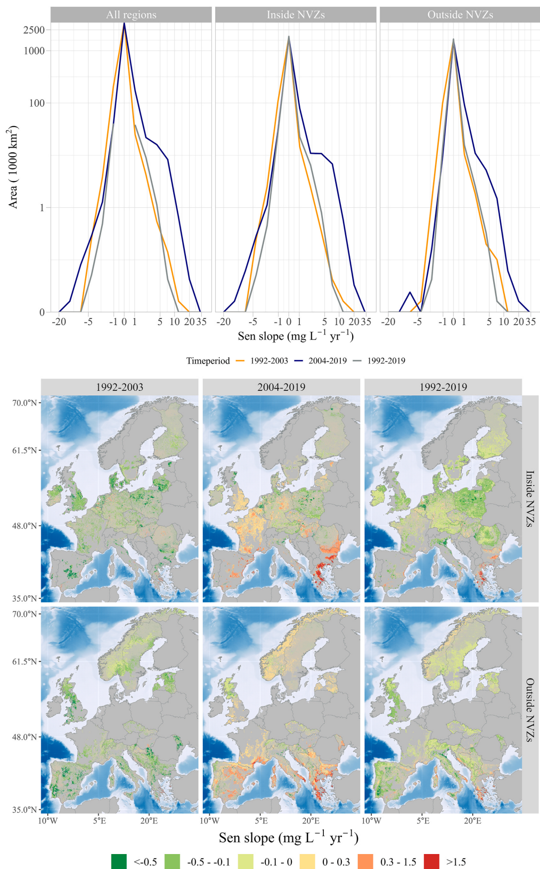
Fig. 4. a) Variability distribution of trends in nitrate concentration in groundwater, per the Sen slope, inside and outside NVZs across three different periods: 1992–2003, 2004–2019 and 1992–2019 using a pseudo logarithmic scale. The spatial distributions (also including all cells) are displayed in b). Non-statistically significant trends are displayed with more transparency.
