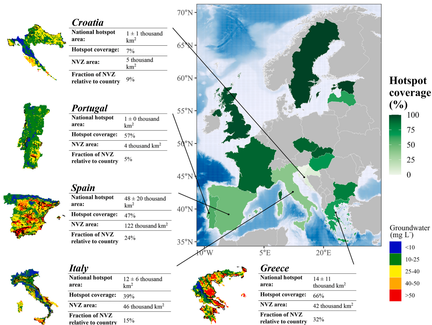
Fig. 7. Hotspot coverage at the national level for MS without a Whole Territory Approach (WTA) implementation for the period 1992–2019. We provide a more detailed analysis for selected countries in Mediterranean Europe with relatively low hotspot coverage and/or large \text{NO}_3^- hotspots: Croatia, Portugal, Spain, Italy and Greece. For each country we also provide the averaged \text{NO}_3^- concentration in groundwater for 1992–2019.
