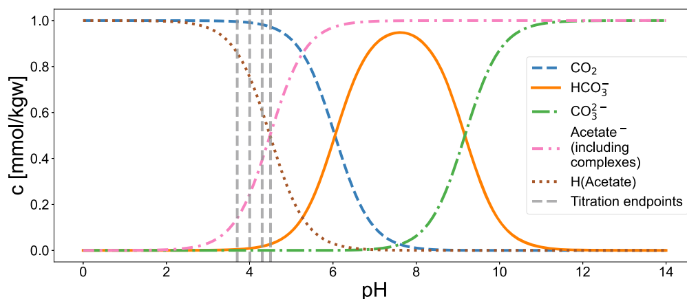
Fig. 7. Acetate (1 mmol NaAcetate) and carbonate (1 mmol NaHCO 3 ) system speciation at T = 25 °C. Modeled with phreeqpython (Heinsbroek, 2021) using the 'minteq.v4.dat' database (US EPAO, 2013) (closed system DIC = 0.001 mol/kg). NaOH is added to the solution to raise the pH, and HCl is added to lower it. The vertical lines indicate the endpoints used for the alkalinity titration [4.5; 4.3; 4.0; 3.7] after (Koenig, 2005).
