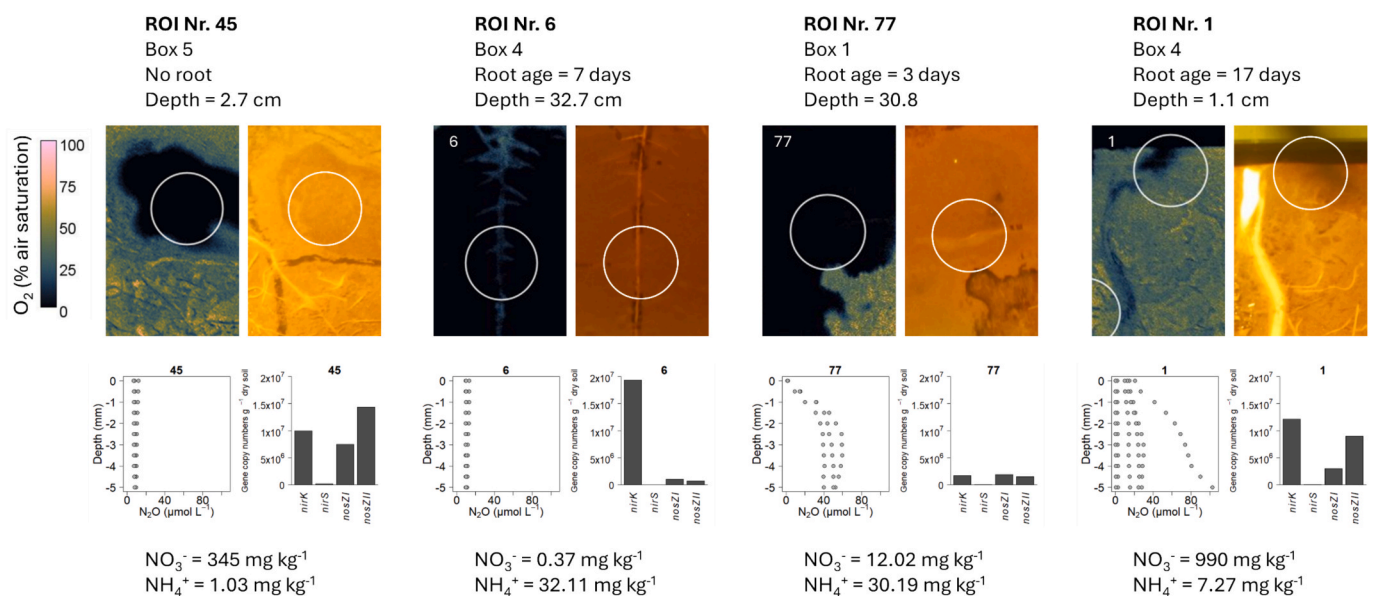
Fig. 5. Characterization of four exemplary ROI at the end of the experiment. False-color image showing O_2 concentration, photo showing root development, N_2O microsensor profiles ( \mu\text{mol } N_2O , depth representing the distance from the optode), bar plot showing gene abundances (gene copy numbers \text{g}^{-1} dry soil), and mineral N content ( \text{mg N kg}^{-1} ). ROI diameter = 16 mm. Root age refers to the days of root growth in the respective ROI.
