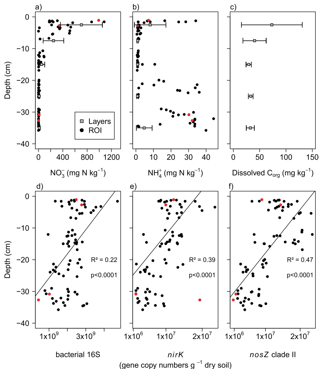
Fig. 4. Depth distribution of (a) NO 3 - , (b) NH 4 + , and (c) DOC content in soil layers and ROI, and (d-f) depth distribution of gene abundances in ROI. Each point represents one of 77 ROI, while grey squares represent mean values \pm standard deviation ( n = 7 ) for different soil layers. Red circles represent ROI Nr. 1, 6, 45, and 77. For gene abundances, regression lines, adjusted R^2 , and p -values of simple linear regressions with depth are depicted.
