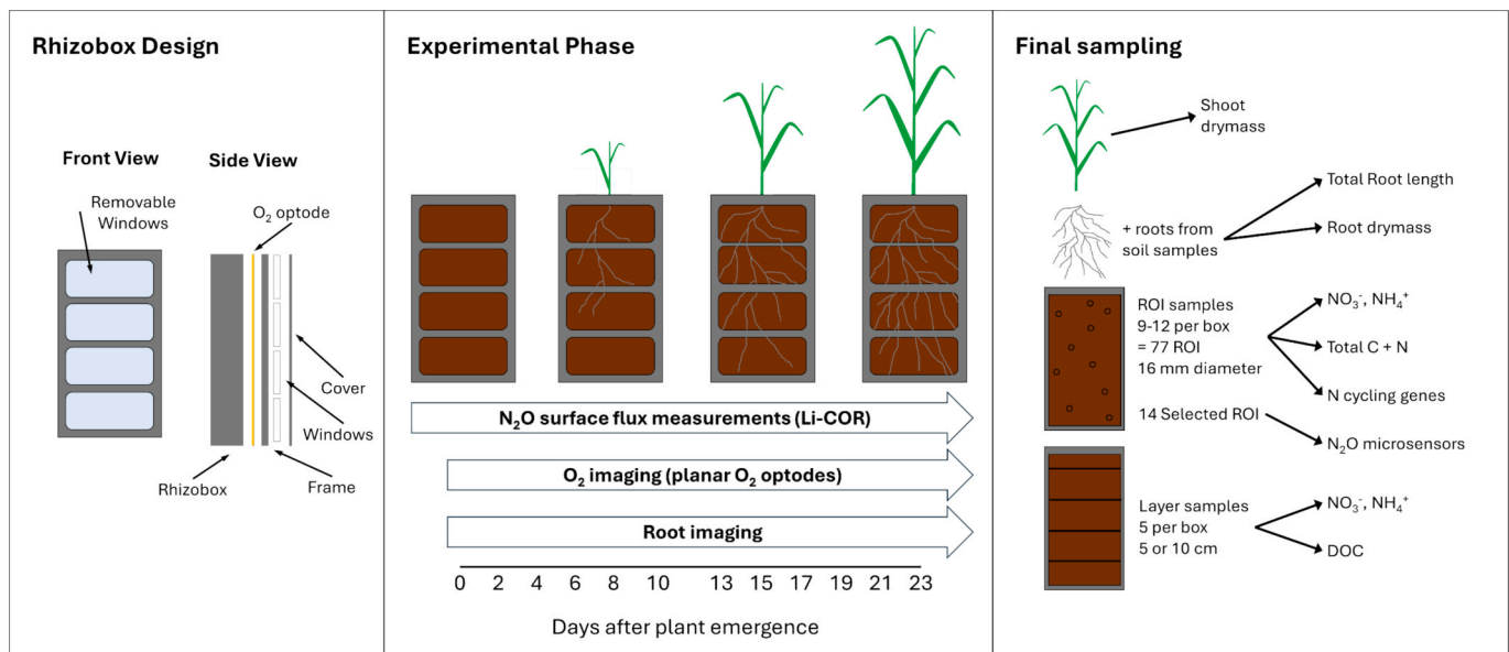
Fig. 1. Schematic overview of rhizobox design, experimental phase, and final sampling of the experiment. The rhizobox covers consisted of an opaque frame with 4 removable window panels. To monitor O_2 concentrations in soil, an O_2 -sensitive optode was attached to the frame before closing the rhizoboxes.
