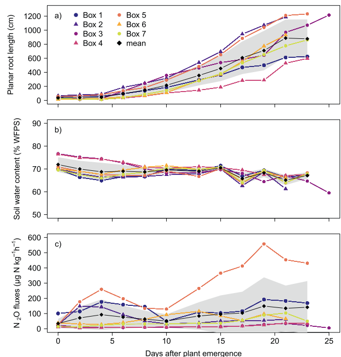
Fig. 2. (a) Planar root length (cm), (b) soil water content (% water-filled pore space), and (c) N 2 O fluxes (µg N 2 O-N kg -1 h -1 ). Colored points and triangles represent each individual rhizobox, black diamonds and grey shaded area represent means ± standard deviation (n = 7).
