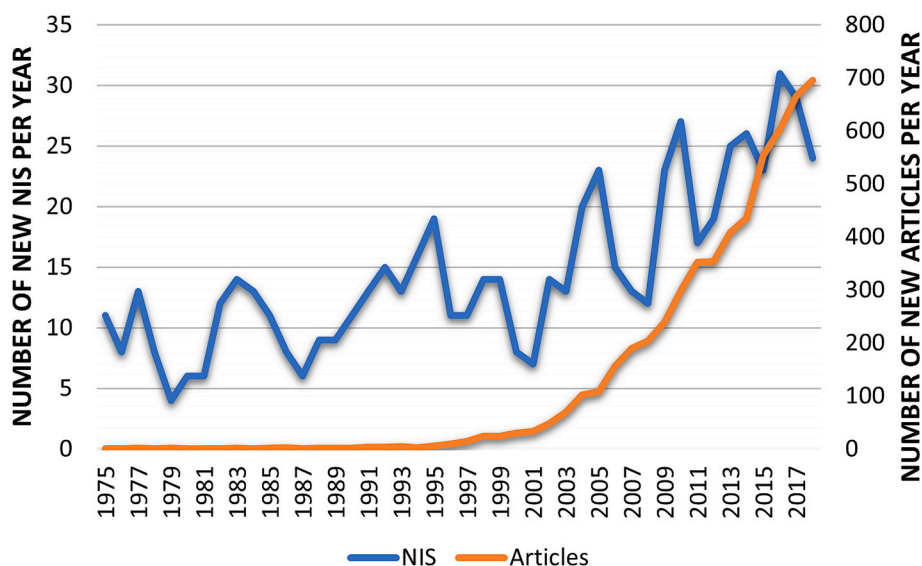
Fig. 9. The annual rates of new NIS introductions and published research articles from 1975 to 2018 using keywords “ Marine invasive species ‘OR’ Marine non-indigenous species ” in Web of Science online platform.
