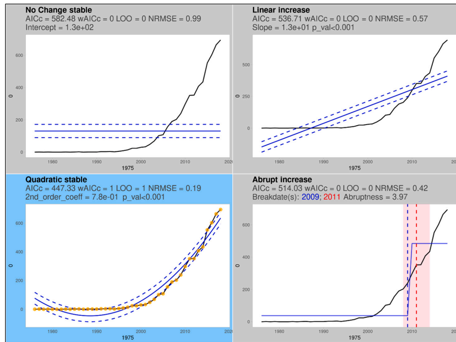
Fig. B.1. Results of the statistical time series analysis for newly published articles from 1975 to 2018 using keywords “Marine invasive species ‘OR’ Marine non-indigenous species ‘OR’ Marine non-native species” in Web of Science online platform.
