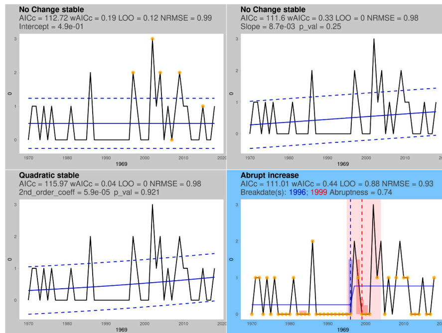
Fig. A.4. Results of the statistical time series analyses for new NIS introductions annually from 1969 to 2018 into the Black Sea. For the abrupt increase model, the blue-labelled year indicates an increasing breakpoint in the annual rate of new NIS, whereas the red-labelled year indicates a decreasing breakpoint. The number of new NIS per year is expressed on the y-axis, while the assessment years (datapoints from 1969 to 2018) are presented on the x-axis. (For interpretation of the references to colour in this figure legend, the reader is referred to the web version of this article.)
