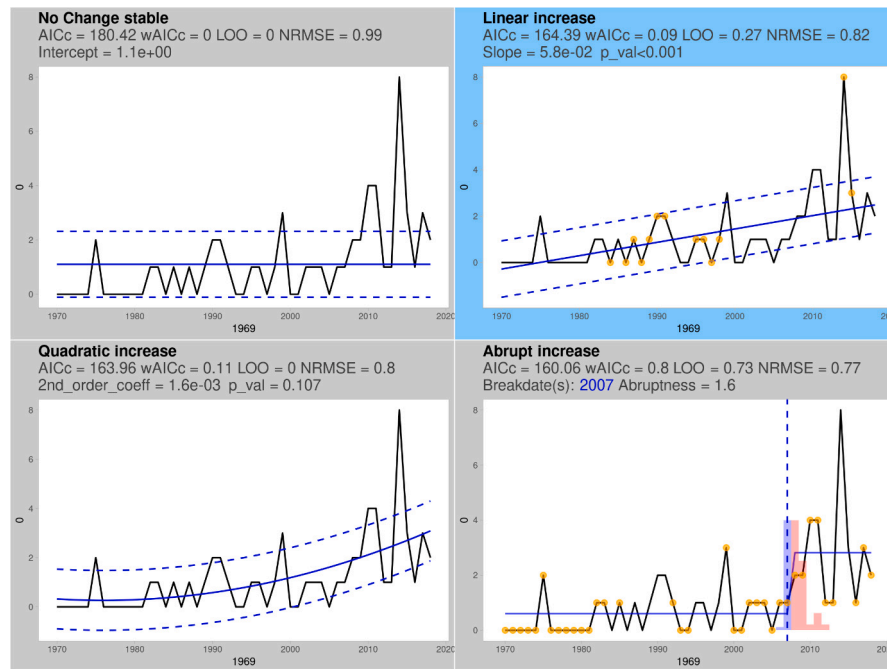
Fig. A.3. Results of the statistical time series analyses for new NIS introductions annually from 1969 to 2018 into the Baltic Sea. For the abrupt increase model, the blue-labelled year indicates an increasing breakpoint in the annual rate of new NIS. The number of new NIS per year is expressed on the y-axis, while the assessment years (datapoints from 1969 to 2018) are presented on the x-axis. (For interpretation of the references to colour in this figure legend, the reader is referred to the web version of this article.)
