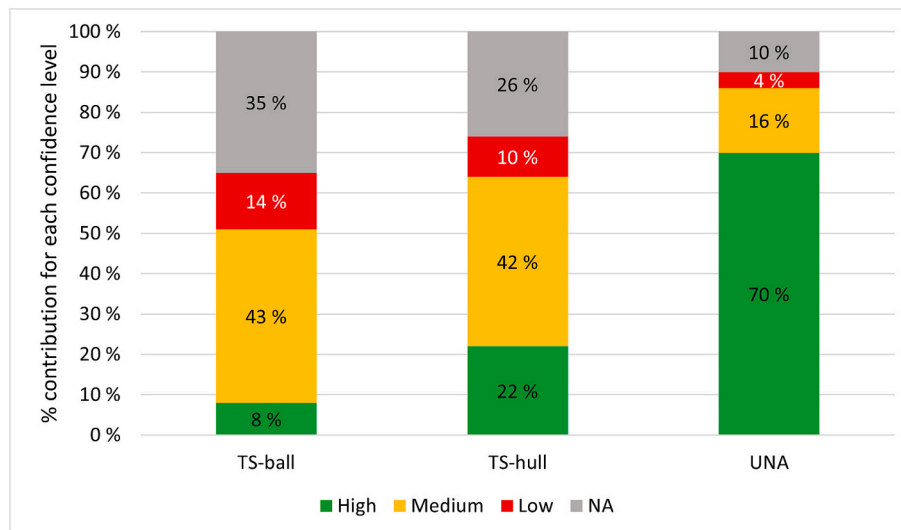
Fig. 6. Percentage contribution of each confidence level category regarding the three most prominent pathways at the Pan-EU level. TS-ball – Transport Stowaway, ballast water, TS-hull – Transport Stowaway, hull fouling, and UNA – Unaided. NA – confidence level for the introduction pathway was not assigned.
