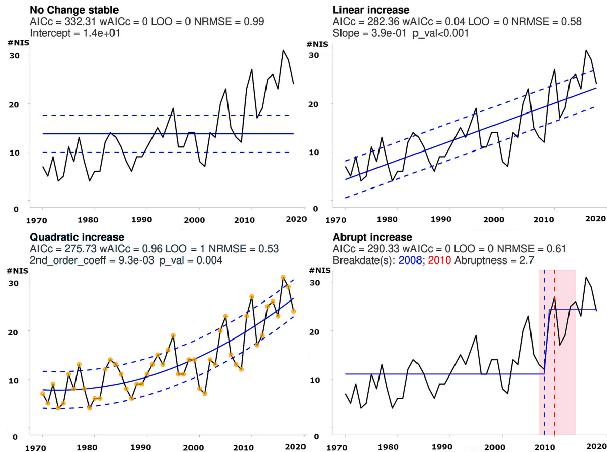
Fig. 3. The statistical time series analyses for the number of new NIS introductions per year at the Pan-EU level from 1969 to 2018. For the abrupt increase model, the blue-labelled year indicates an increasing breakpoint, whereas the red-labelled year indicates a decreasing breakpoint in the rate of new NIS introductions. (For interpretation of the references to colour in this figure legend, the reader is referred to the web version of this article.)
