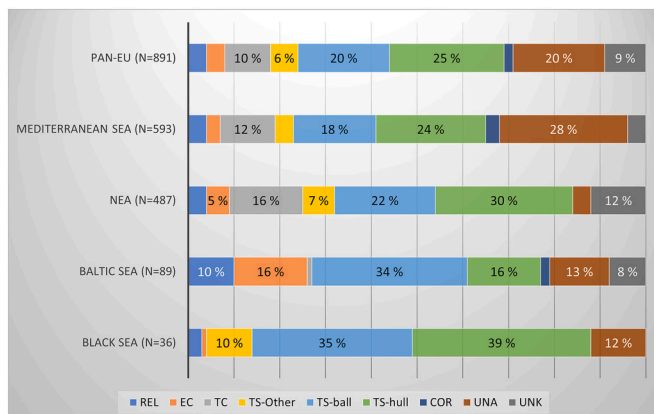
Fig. 5. Percentage contribution of introduction pathways into the EU and regional seas until 2021. REL – Release in Nature, EC – Escape from Confinement, TC – Transport Contaminant, TS – Transport Stowaway (divided into TS-ball, TS-other and TS-hull), COR – Corridor, UNA – Unaided, and UNK – Unknown. Data labels (% contribution) are provided only for the pathways that contributed \geq 5\% to the NIS introductions for each study region. NEA – North-East Atlantic Ocean.
