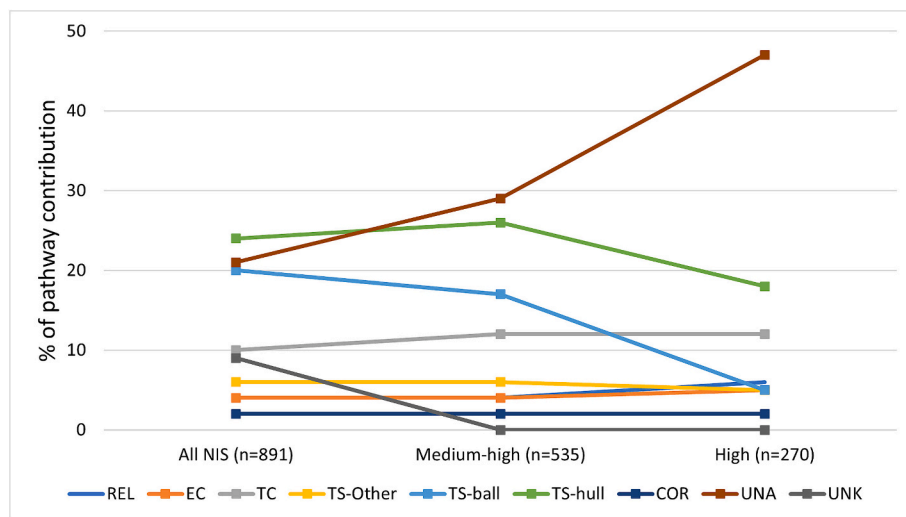
Fig. 8. Percentage contribution of introduction pathways into the EU for all NIS (left) compared to only those NIS with high or medium (middle), and only those NIS with high confidence level pathway designation (right). REL – Release in Nature, EC – Escape from Confinement, TC – Transport Contaminant, TS – Transport Stowaway (divided into TS-ball, TS-other and TS-hull), COR – Corridor, UNA – Unaided, and UNK – Unknown.
