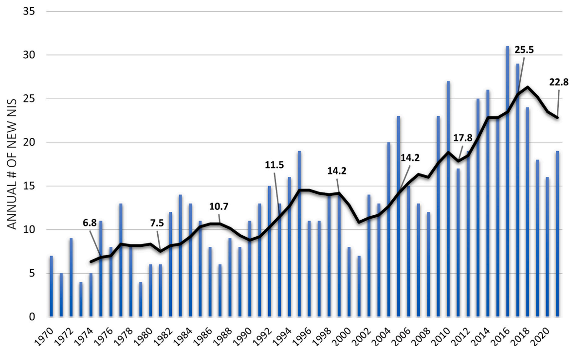
Fig. 2. The annual rate of new NIS introductions to EU seas from 1970 to 2021. The blue columns represent the annual rates of new NIS, and the black line represents moving annual averages for all six-year periods across the study years. The data labels within the moving average refer to the last year of each fixed six-year assessment period provided by Tsiamis et al. (2021) with the exception that the most recent data label (22.8) is an annual average from a period of 2016–2021 (the most recent six-year assessment period available for this study). (For interpretation of the references to colour in this figure legend, the reader is referred to the web version of this article.)
