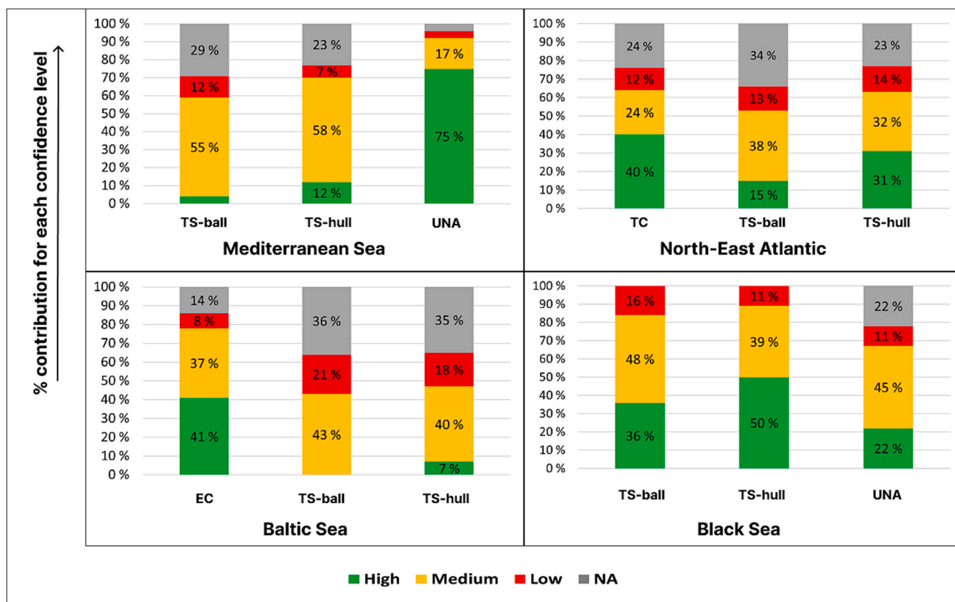
Fig. 7. Confidence levels for the most prominent NIS pathways into EU regional seas until 2021. TC – Transport Contaminant, TS-ball – Transport Stowaway ballast water, TS-hull – Transport Stowaway hull fouling, UNA – Unaided, and EC – Escape from Confinement. NA – level of confidence for the pathway designation was not assigned. Data labels (% contribution) are provided only for the confidence levels that contributed \geq 5\% for each of the presented pathway assessments.
