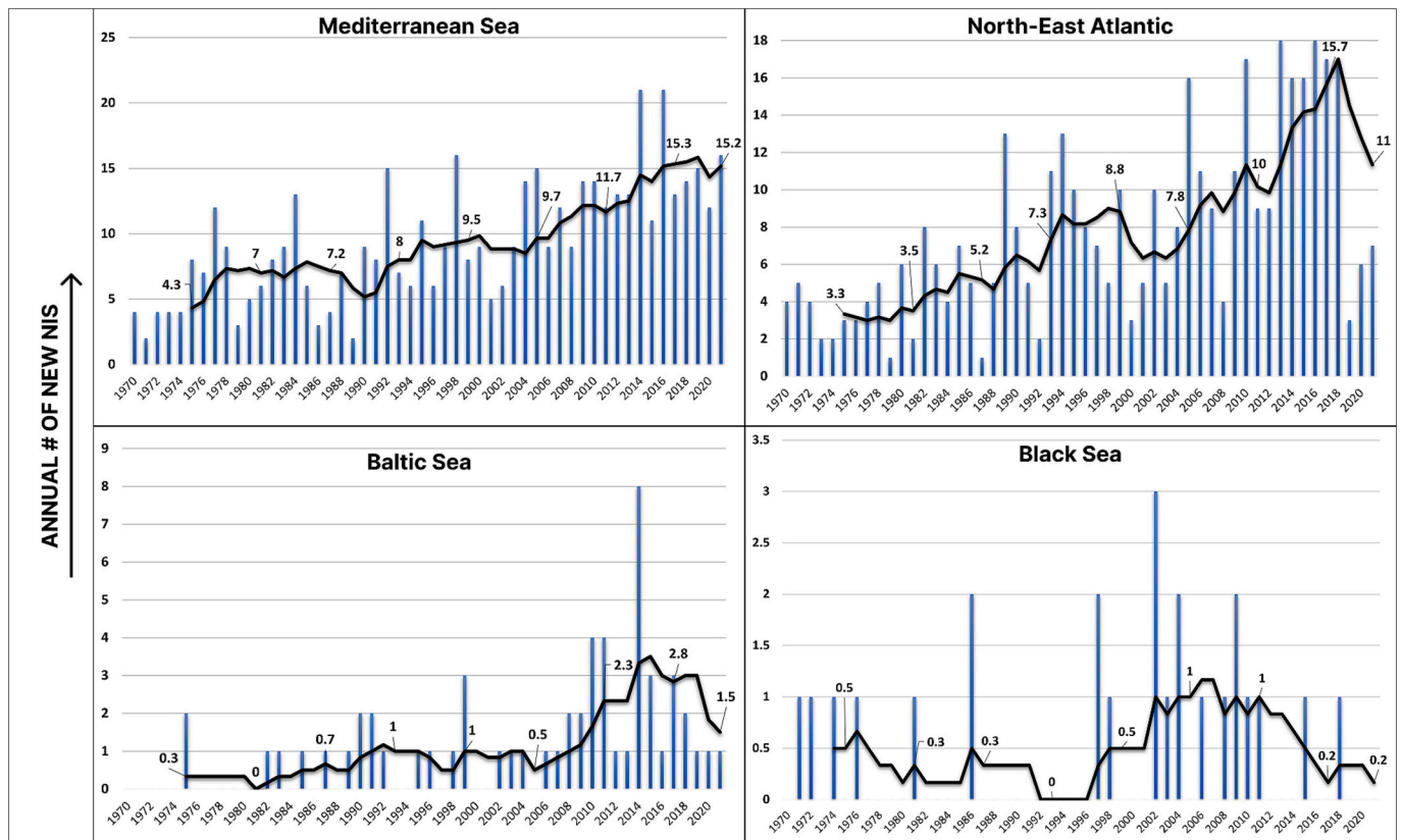
Fig. 4. The annual rate of new NIS introductions to European regional seas from 1970 to 2021. The blue columns represent the annual rates of new NIS, and the black line represents moving annual averages for all six-year periods across the study years. The data labels within the moving average refer to the last year of each fixed six-year assessment period provided by Tsiamis et al. (2021) with the exception that the most recent data labels are annual averages from a period of 2016–2021 (the most recent six-year assessment period available for this study). (For interpretation of the references to colour in this figure legend, the reader is referred to the web version of this article.)
