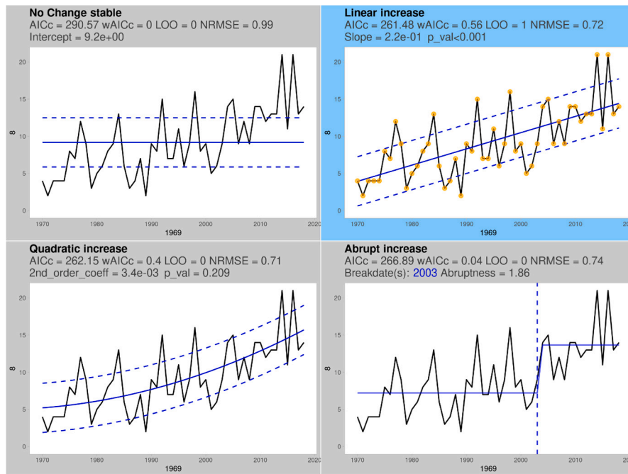
Fig. A.1. Results of the statistical time series analyses for new NIS introductions annually from 1969 to 2018 into the Mediterranean Sea. For the abrupt increase model, the blue-labelled year indicates an increasing breakpoint in the annual rate of new NIS. The number of new NIS per year is expressed on the y-axis, while the assessment years (datapoints from 1969 to 2018) are presented on the x-axis. (For interpretation of the references to colour in this figure legend, the reader is referred to the web version of this article.)
