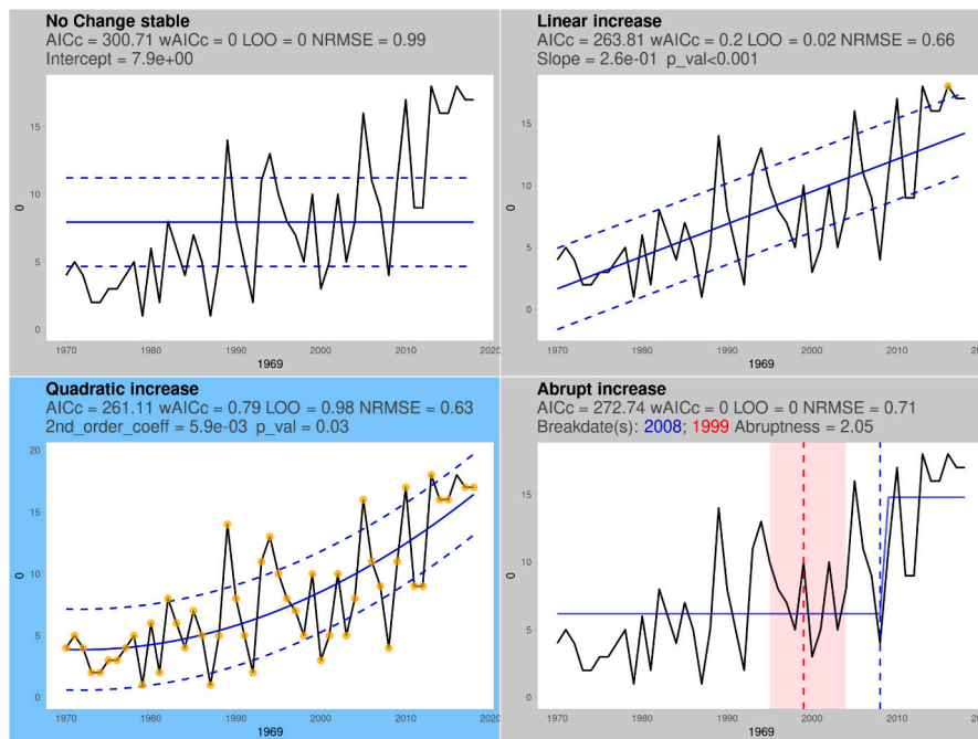
Fig. A.2. Results of the statistical time series analyses for new NIS introductions annually from 1969 to 2018 into the North-East Atlantic Ocean. For the abrupt increase model, the blue-labelled year indicates an increasing breakpoint in the annual rate of new NIS, whereas the red-labelled year indicates a decreasing breakpoint. The number of new NIS per year is expressed on the y-axis, while the assessment years (datapoints from 1969 to 2018) are presented on the x-axis. (For interpretation of the references to colour in this figure legend, the reader is referred to the web version of this article.)
