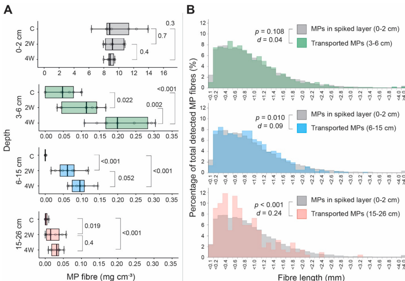
Fig. 3. Depth-dependent mass and length distributions of MP fibres. (A) Including control columns (C: no earthworms), and in bioturbation columns sampled after 2 and 4 weeks (2 W, 4 W). Boxplots represent the interquartile range (IQR), where the median is represented as a vertical bar and points showing the individual data points ( n = 9 ). Horizontal error bars indicate the range excluding outliers (1.5 times IQR). (B) Length distribution of transported MP fibres in comparison to the initial size distribution. Displayed numbers are p -values based on Welch's t -tests comparing the length of all detected MPs; d -values represent the calculated Cohen's d indicating effect magnitude.
