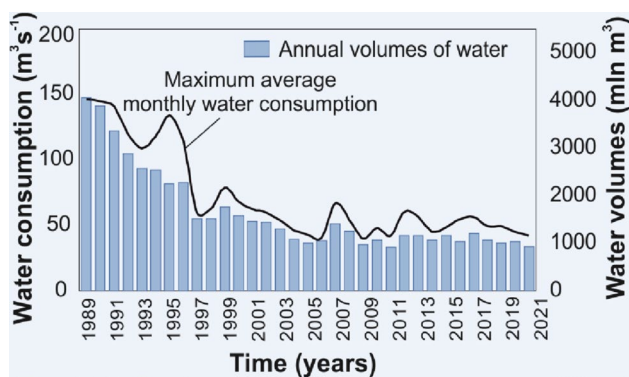
Fig. 4 Annual volumes of water (million m 3 ) and maximum average monthly water consumption (m 3 /s) supplied for the Zaporizhzhia TPP and NPP and other enterprises and cities, from the Kakhovka reservoir
