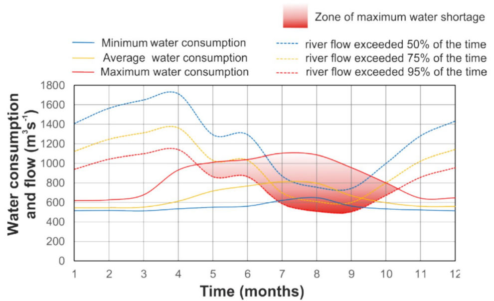
Fig. 10 Intra-annual distribution of water inflow ( m^3/s ) to the Kakhovka reservoir for years taking into account scenarios with different levels of water availability in and different needs from the reservoir, and the need to support aquatic ecosystems south of the reservoir (i.e. south of the Kakhovka HPP)
