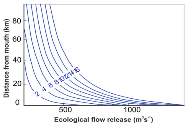
Fig. 8 Nomogram for determining the length of the wedge of salt water in the Dnipro estuary (km) at different water flow rates ( \text{m}^3/\text{s} ) and initial salinity concentration (%o, numbers on the lines). Based on the data from Oksiyuk et al. 1997
