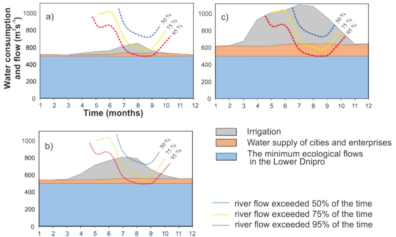
Fig. 11 Intra-annual distribution of water supplied to or consumed by different actors, taking into account scenarios with different water inflow ( m^3/s ) into the Kakhovka reservoir for years with 50, 75, and
