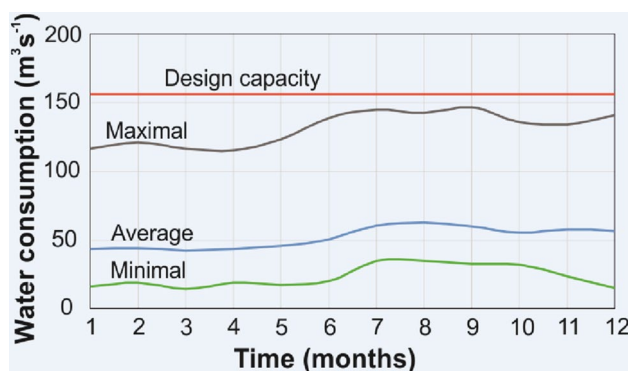
Fig. 3 Multi-year average intra-annual distribution of water consumption (m 3 /s) from the Kakhovka reservoir made available to water consumers including the needs of the Zaporizhzhia TPP and NPP and other enterprises and settlements
