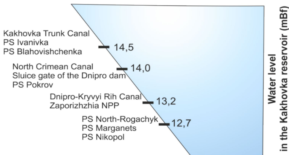
Fig. 9 Minimal level of water needed for the proper operation of different hydraulic structures, such as irrigation canals and water intakes for various consumers in the pre-war period. Based on data from Yatsyk et al. 2003. PS pumping station
