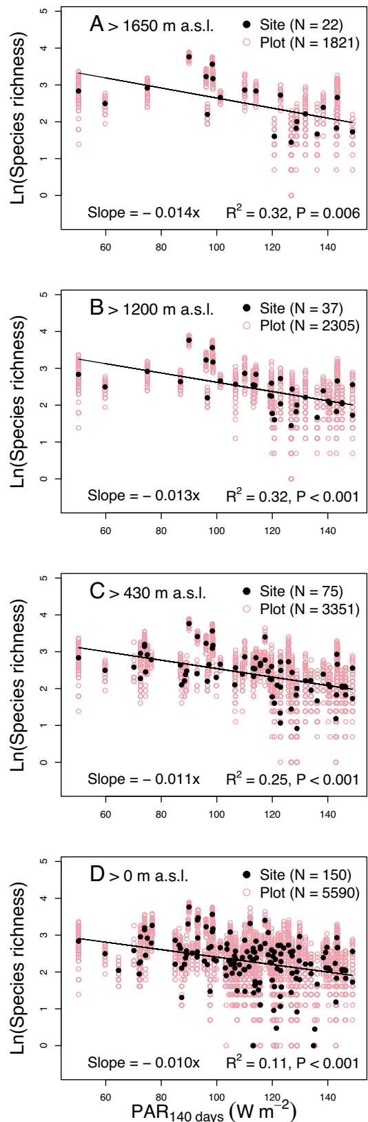
Fig. 1. Relationship between the log-transformed plant species richness and the mean PAR during the 140-day period of highest PAR ( \text{PAR}_{140 \text{ day}} ). The relationship is shown across sites at >1,650 m a.s.l. (A), at >1,200 m a.s.l. (B), at >430 m a.s.l. (C), and at >0 m a.s.l. (all sites; D). \text{PAR}_{140 \text{ day}} was calculated based on 22 y of observation. The linear models were calculated based on the site-level data (and not based on the plot-level data, which are shown to give insight into the within-site variability). The sites were divided into different elevation categories by repeated binary splits. N indicates the number of observations.
