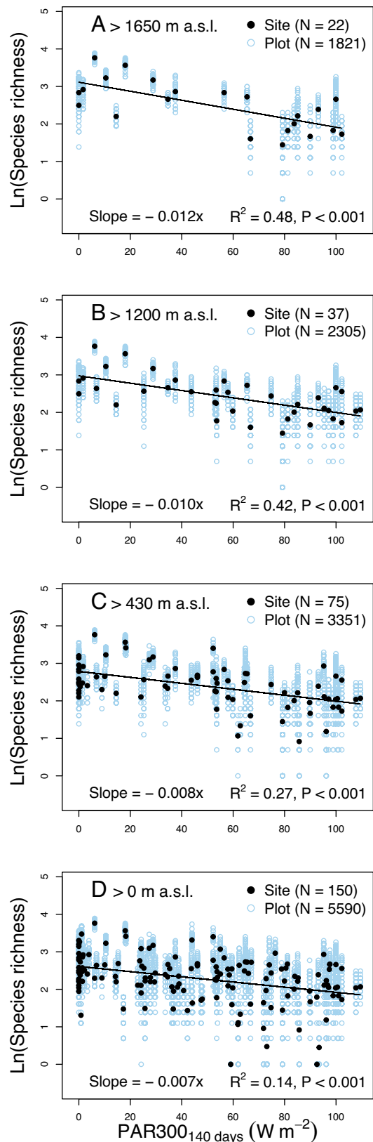
Fig. 2. Relationship between the log-transformed plant species richness and intense PAR during the 140-day period of highest PAR ( PAR_{300,140 \text{ days}} ). PAR_{300,140 \text{ days}} is calculated as the mean PAR during the 140-day period of highest PAR after setting all 3-h periods with PAR < 300 to 0 \text{ W m}^{-2} based on 22 y of observation. The relationship is shown across sites at >1,650 m a.s.l. (A), at >1,200 m a.s.l. (B), at >430 m a.s.l. (C), and at >0 m a.s.l. (all sites; D). The sites were divided into different elevation categories by repeated binary splits. The linear models were calculated based on the site-level data (and not based on the plot-level data, which are shown to give insight into the within-site variability).
