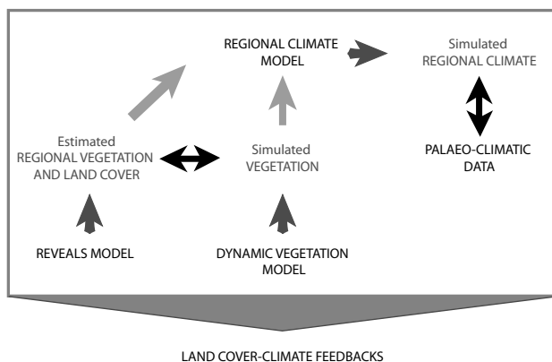
Fig. 9. Model-data comparison scheme for the LANDCLIM project. The simple arrows represent model inputs or outputs. The double arrows represent the model-data comparison steps. REVEALS model (Sugita 2007a); dynamic vegetation model= LPJ-GUESS (Smith et al., 2001); regional climate model=RCA3 (Kjellström et al., 2005). For details, see text.
