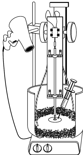
Figure 3. Assembled spinning disc equipment. The bowl has a cut-out in the illustration to show the placement of the disc, the two nozzles for compressed air and the seed lot being coated. The application of the coating material was done by hand using the syringe to put drops of material solution or emulsion onto the spinning disc. (Used in coating rape seed. See Paper III. A slightly modified version was used in coating wheat kernels with lacquer. See Paper II.)
