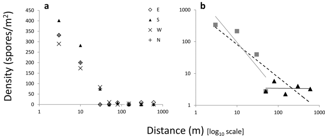
Figure 2. The estimated spore densities, based on the observed number of colonised pots, at different distances. a. Spore densities (on a linear scale) for the four cardinal directions (distances on a logarithmic scale). b. The mean spore densities at each distance (in log-log space). Power trend lines are shown both for the full data (hatched) and for distances within and beyond 40–50 m separately. The regression coefficients b are -1.032 for the full data set (5–600 m), -1.563 for 5 to 50 m and -0.012 for 50 to 600 m. doi:10.1371/journal.pone.0041987.g002
