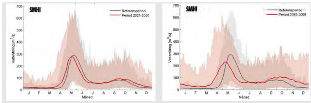
Figure 34. Average water flow in the Ångermanälven during the months of the year for the reference period 1963-1992 compared to the predicted future 2021-2050 (from Länsstyrelsen Västerbotten 2011).
