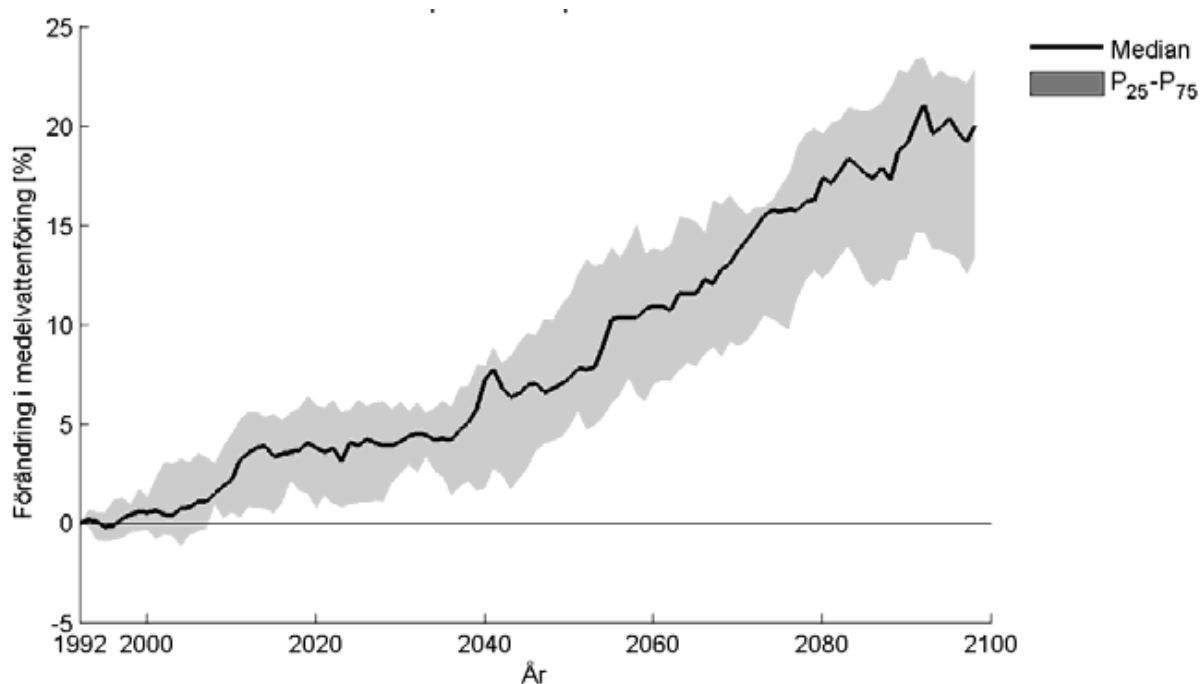
Figure 35. Percentage change in total average annual runoff in Ångermanälven, outlet Malmomaj, for 16 climate simulations (12 for 2050) relative to the reference period 1963-1992. Each year's value consists of a median (black line) taken over the preceding 30 years (for example, the value is 2050 mean of the period 2021-2050 compared with the mean 1963 - 1992). The gray area shows the variation between the 25th and 75th percentiles (from Länsstyrelsen Västerbotten 2011).
