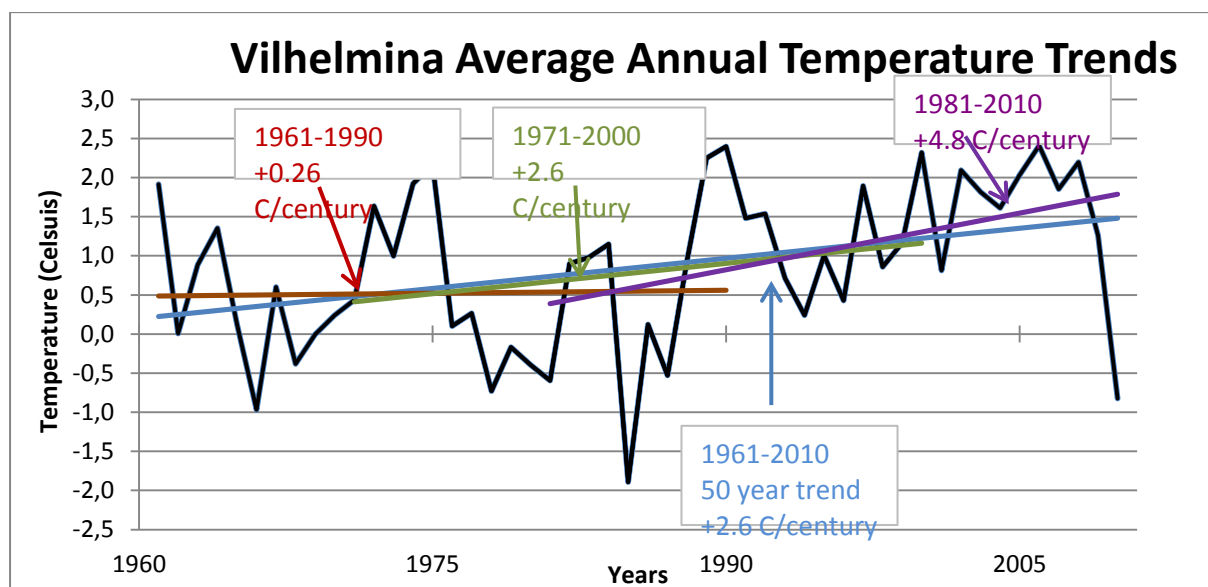
Figure 4. Vilhelmina average annual temperature with 30 year trend lines and 50 year trend line from 1961 to 2010 (raw data from SMHI 2012 for Vilhelmina GPS location from Sveriges länsstyrelser 2012).
