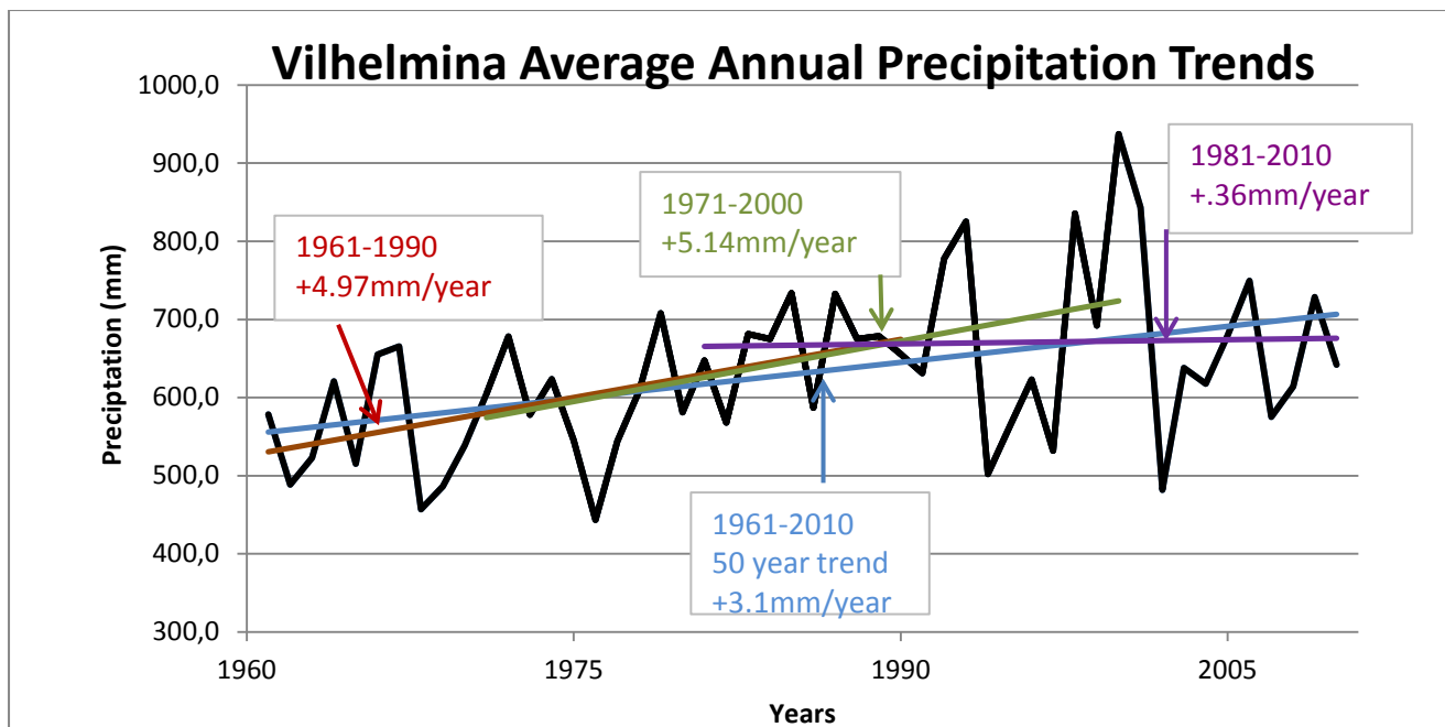
Figure 5. Vilhelmina average annual precipitation with 30 year trend lines and 50 year trend line from 1961 to 2010 (raw data from SMHI 2012 for Vilhelmina GPS location from Sveriges länstyrelser 2012).
