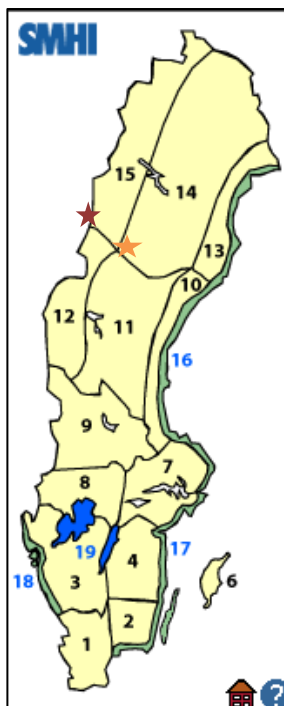
Figure 3. The division into districts based on SMHI's forecast districts. Vilhelmina Municipality is located in District 14 and 15, Vilhelmina town is marked with an orange star, and Stekenjokk is marked with a dark red star (from Rossby Centre 2012).
