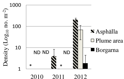
Figure 4. Increasing density over time of M. leucophaeata on artificial substrate plates deployed at three sites (mean \pm SD). * = No mussels present. ND = no data.
