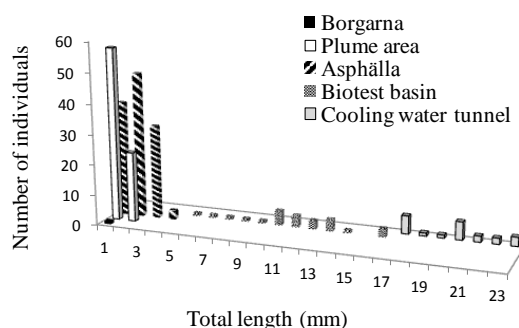
Figure 5. Length distribution of the M. leucophaeata encountered in vicinity of the Swedish nuclear power plant in the Southern Bothnian Sea.
