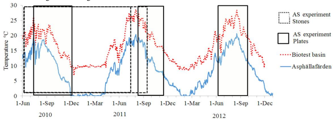
Figure 2. Temperature in Asphällafjärden (blue solid line) and Biotest basin (red dotted line) recorded by automatic data loggers from 1 June 2010 to 31 December 2012. Time of artificial substrate experiment using stones is shown by the dashed-line blocks while experiments conducted using Plexiglass plates is indicated by solid-line blocks.
