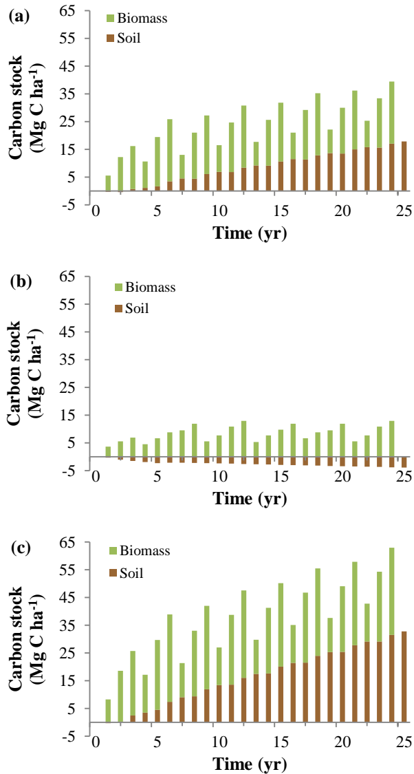
Fig. 8 Carbon (C) stored in willow biomass (stems, leaves, roots) and soil each year during 25 years of cultivation on agricultural land previously used as green fallow in (a) the Base scenario, (b) the Low yield scenario and (c) the High yield scenario. Net change compared with baseline year zero (previous land use), i.e. negative values indicate decreased carbon stock and positive values increased carbon stock compared with the previous land use. Carbon in litter was assumed to enter the soil pool with a one-year delay.
