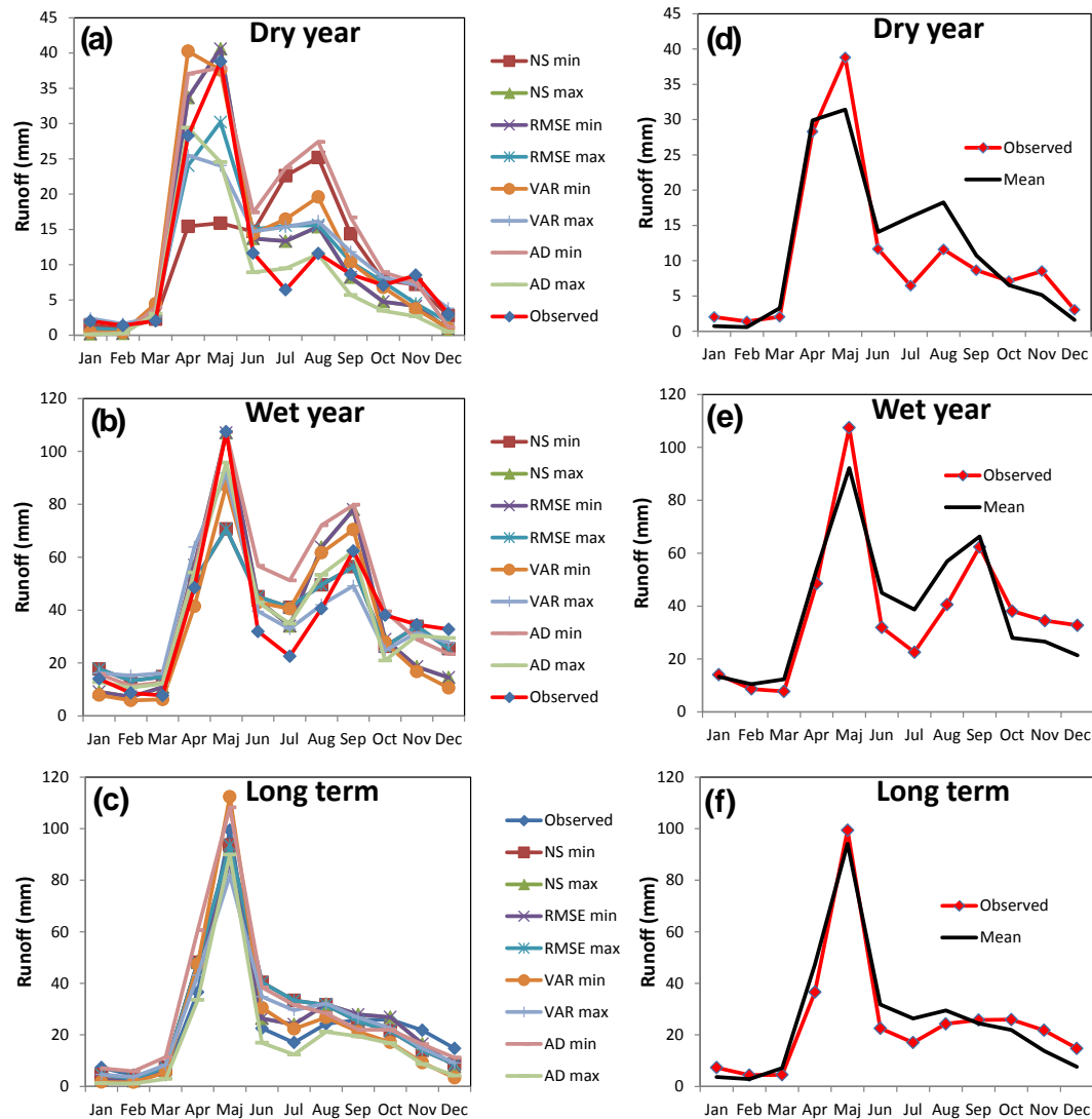
Figure 5. Summary plots showing the prediction ranges of seasonal runoff dynamics of behavioural parameter sets using different performance metrics in (a) dry years, (b) wet years and the (c) long term. (d) to (f) show the corresponding model performances using the behavioural means of the metrics in (a) to (c).
