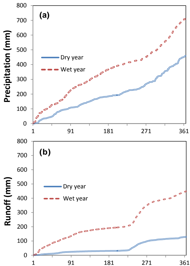
Figure 2. Cumulative plots of (a) precipitation and (b) runoff in dry (1995, 2002, 2005 and 2010) and wet (1987, 1992, 2000 and 2001) hydrologic years. The hydrologic year is 1 September (day 1) to August 31 of the following year (day 365). The cumulative plots shown here represent the average for all the dry and wet years noted above.
