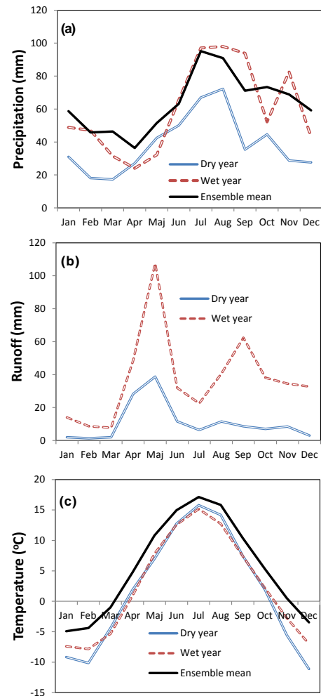
Figure 3. Seasonal patterns of (a) present-day precipitation in dry and wet years vs. the ensemble mean (bias-corrected) of future precipitation projections, (b) present-day runoff dynamics in dry and wet years and (c) present-day temperature in dry and wet years relative to the ensemble mean (bias-corrected) of future temperature projections. Note that the dry and wet years in these plots represent the average of all the individual dry and wet years, respectively.
