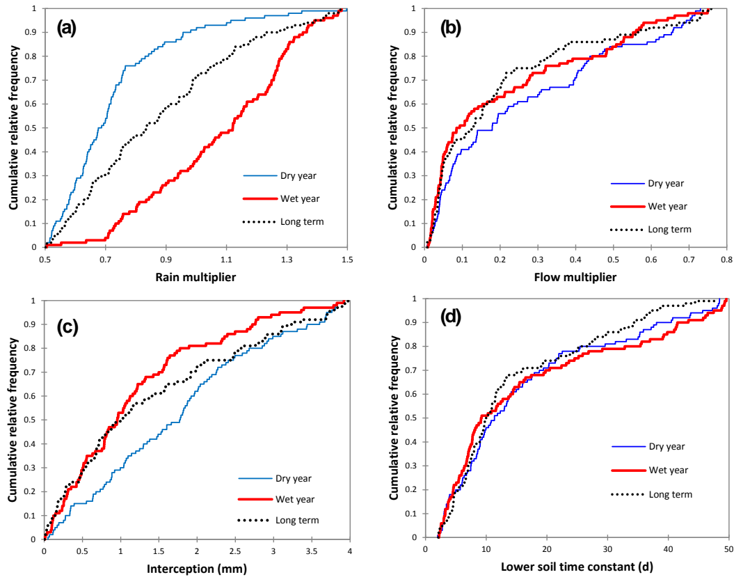
Figure 6. Cumulative distribution function (CDF) of behavioural parameters (top 100 iterations from the Monte Carlo runs) in wet and dry years vs. the long-term record. (a) is the rain multiplier, (b) is the flow multiplier, (c) is the interception and (d) is the lower soil time constant in the lower soil box. A rectangular distribution (straight line plot) defines parameter behaviours that were not sensitive (not left- or right-skewed).
