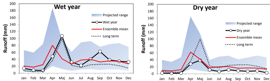
Figure 8. Example of the range of runoff projection using wet year parameterization that closely depicts the future vs. projected range based on dry year parameterization. The projected range was simulated to constrain uncertainty in extreme wet and dry conditions in the future using the behavioural parameter sets (top 100 iterations from MCMC) for each of the 15 RCM scenarios (100 parameters by 15 RCMs = 1500 runs each for dry and wet years). The ensemble mean represents the mean of the 1500 realizations, while long term depicts the mean of the long-term series.
