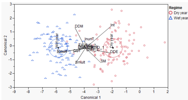
Figure 7. Separation of the behavioural parameter sets (top 100 iterations from MCMC) in the dry and wet year hydrologic regimes using discriminant function analysis (DFA). Wet and dry year hydrology separated mainly on parameters related to evapotranspiration (DDE), interception (Int) and rain multiplier (Rmult) on canonical 1. Parameters were separated on snow multiplier (Smult), snowmelt (SM) and degree day melt factor (DDM) on canonical 2. The circles represent normal 50% contours. Parameters are defined in Table 3.
