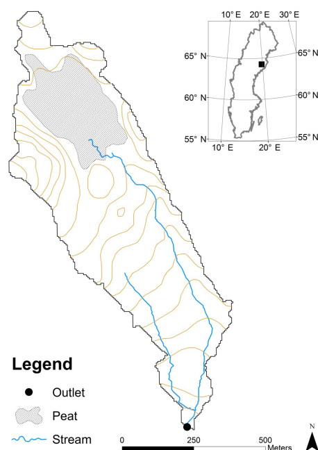
Figure 1. Svartberget, a long-term monitored headwater catchment in the northern boreal ecozone of Sweden. The catchment (50 ha) drains terrestrial area consisting of forest (82 %) and upland mire (18 %). Streamflow measurements were taken at the downstream confluence point.
