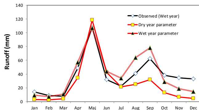
Figure 4. Quantification of predictive uncertainty in runoff simulations when the best parameter set (based on NS) calibrated for dry years was used for wet year observed series.
