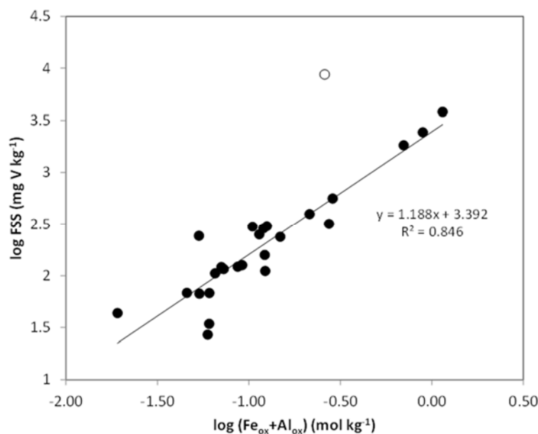
Fig. 5. Log-log relationship between the amount of oxalate-extractable Fe and Al ( \text{Fe}_{\text{ox}} + \text{Al}_{\text{ox}} ) and the FSS (i.e. the amount of V sorbed at [\text{V}] = 2.5 \text{ mg L}^{-1} ). The empty circle, which represents the sample from Örbyhus 2, was removed from the regression (see text).
