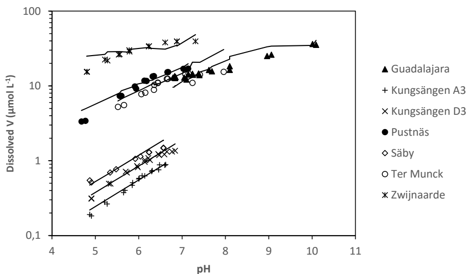
Fig. 3. Dissolved V as a function of pH for seven soils, after the addition of 150 \mu\text{mol L}^{-1} vanadate(V). The symbols represent observations whereas the lines are Freundlich model fits with \eta = 0.36 .
