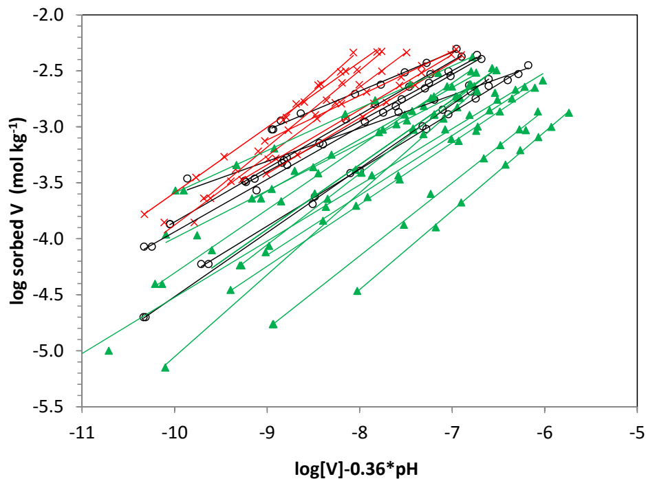
Fig. 4. Amount of sorbed V as a function of the term \log [V]-0.36 \cdot \text{pH} for all 26 soils of the study. Samples are grouped according to the content of oxalate-extractable Al and Fe content. Red crosses represent samples with \text{Fe}_{\text{ox}}+\text{Al}_{\text{ox}} > 0.2 \text{ mol kg}^{-1} , black circles are soils with \text{Fe}_{\text{ox}}+\text{Al}_{\text{ox}} ranging from 0.1 to 0.2 \text{ mol kg}^{-1} , and green triangles are soils with \text{Fe}_{\text{ox}}+\text{Al}_{\text{ox}} < 0.1 \text{ mol kg}^{-1} . Model fits are shown as solid lines.
