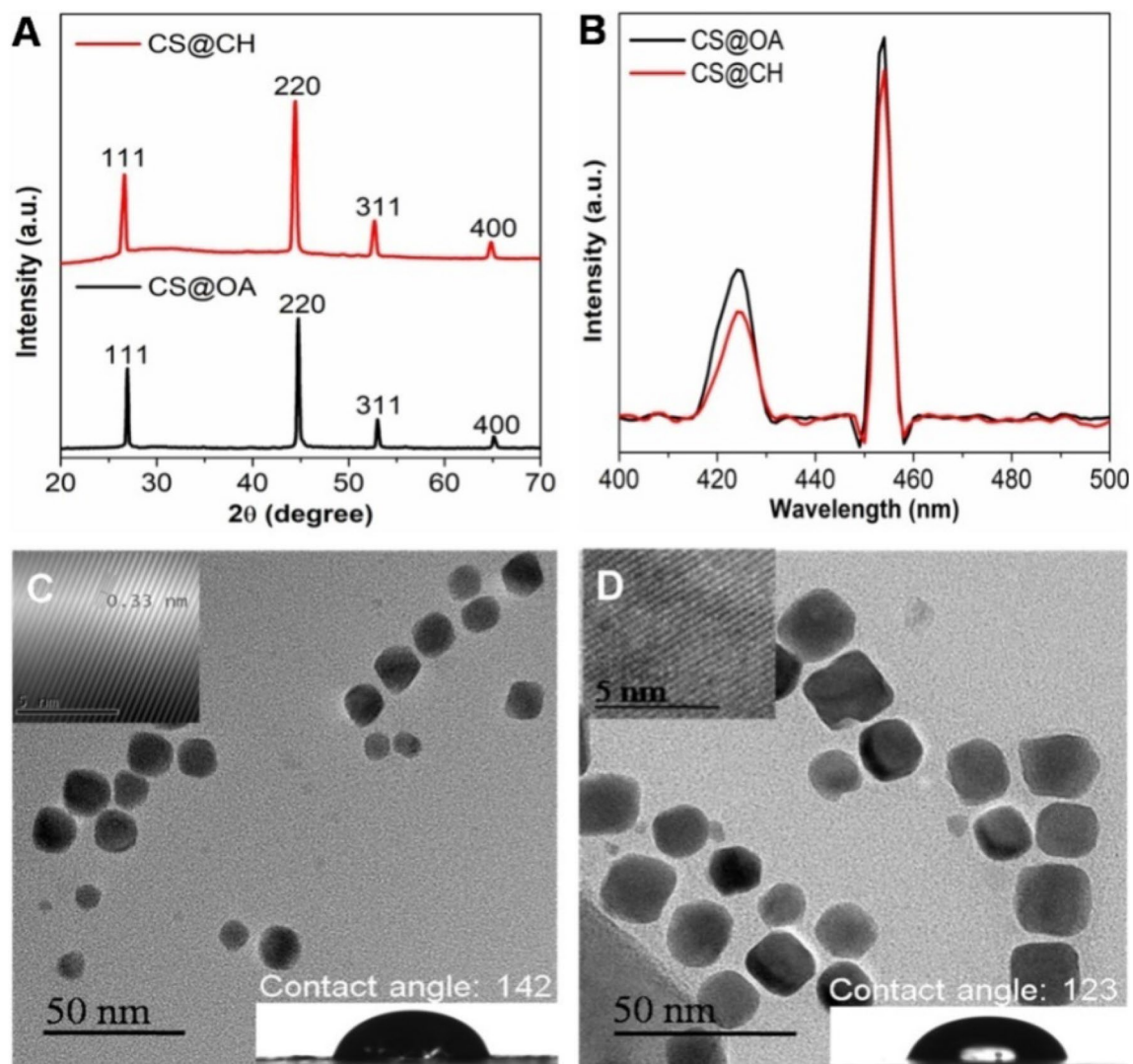
Figure 1. Characterization of the \text{Cu}_{2-x}\text{Se} NPs (as-prepared oleylamine-coated CS@OA and chitosan-coated CS@CH). (A) XRD patterns of CS@OA (black curve) and CS@CH NPs (red curve). (B) PL spectra of CS@OA (black curve) and CS@CH (red curve) recorded at a 370 nm excitation wavelength. (C,D) TEM images of CS@OA and CS@CH showing the \text{Cu}_{2-x}\text{Se} NPs, respectively (inset (top left corner): HR-TEM images of the CS@OA and CS@CH NPs showing a 0.33 nm lattice spacing, corresponding to the (111) plane of \text{Cu}_{2-x}\text{Se} ) (inset (bottom right corner): contact angle on glass substrates coated with CS@OA or CS@CH NPs).
